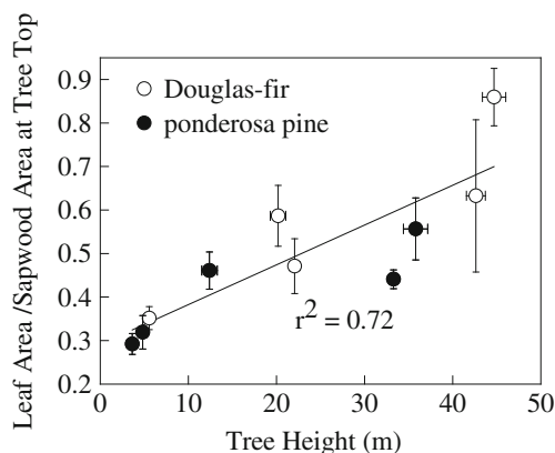
Fig. 2 Leaf area/sapwood area (in \text{m}^{-2} \text{cm}^{-2} ) at node 15 from tree top versus tree height for Douglas-fir and ponderosa pine trees (each point shows mean \pm s.e. for n=5-6 samples)
