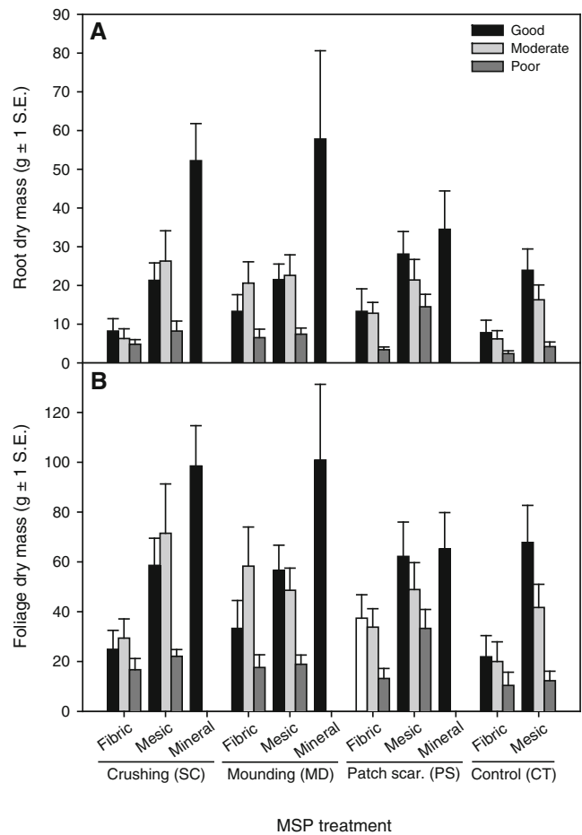
Fig. 3 Root (a) and foliage (b) dry mass of planted black spruce seedlings by MSP treatment, substrate type and drainage
