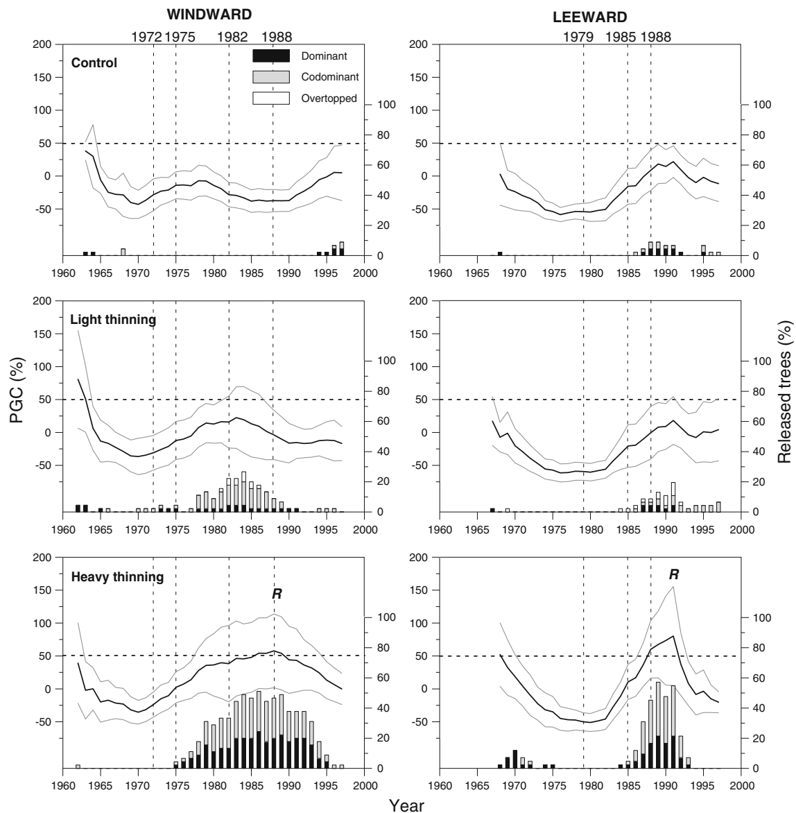
Fig. 3 Mean (black lines) and standard deviation (grey lines) of percentage growth change (PGC) for BAI of trees by treatment and slope. Horizontal dashed lines Minimum threshold (50% PGC) for release detection, R highest PGC above the threshold, bars percentage
