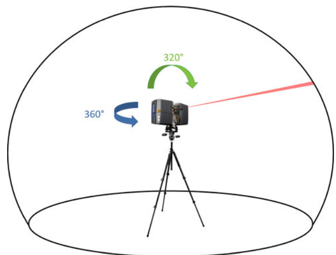
Fig. 1 Operating principle of a terrestrial LiDAR (light detection and ranging) scanner (FARO Photon 120). A laser beam deflected by a rotating mirror scans a vertical plane, and the complete rotation of the device allows hemispherical scanning. This results in the digitisation and the representation of surrounding objects in a three-dimensional (3D) point cloud
