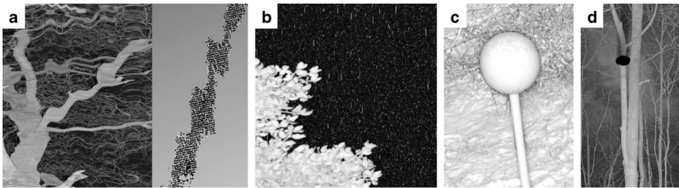
Fig. 4 Impact of climatic and sky conditions on scan quality. Wind leads to poor descriptions of tree axes ( a ), whereas snow intercepts laser beams and leads to an increase of noise points ( b ) and poor
