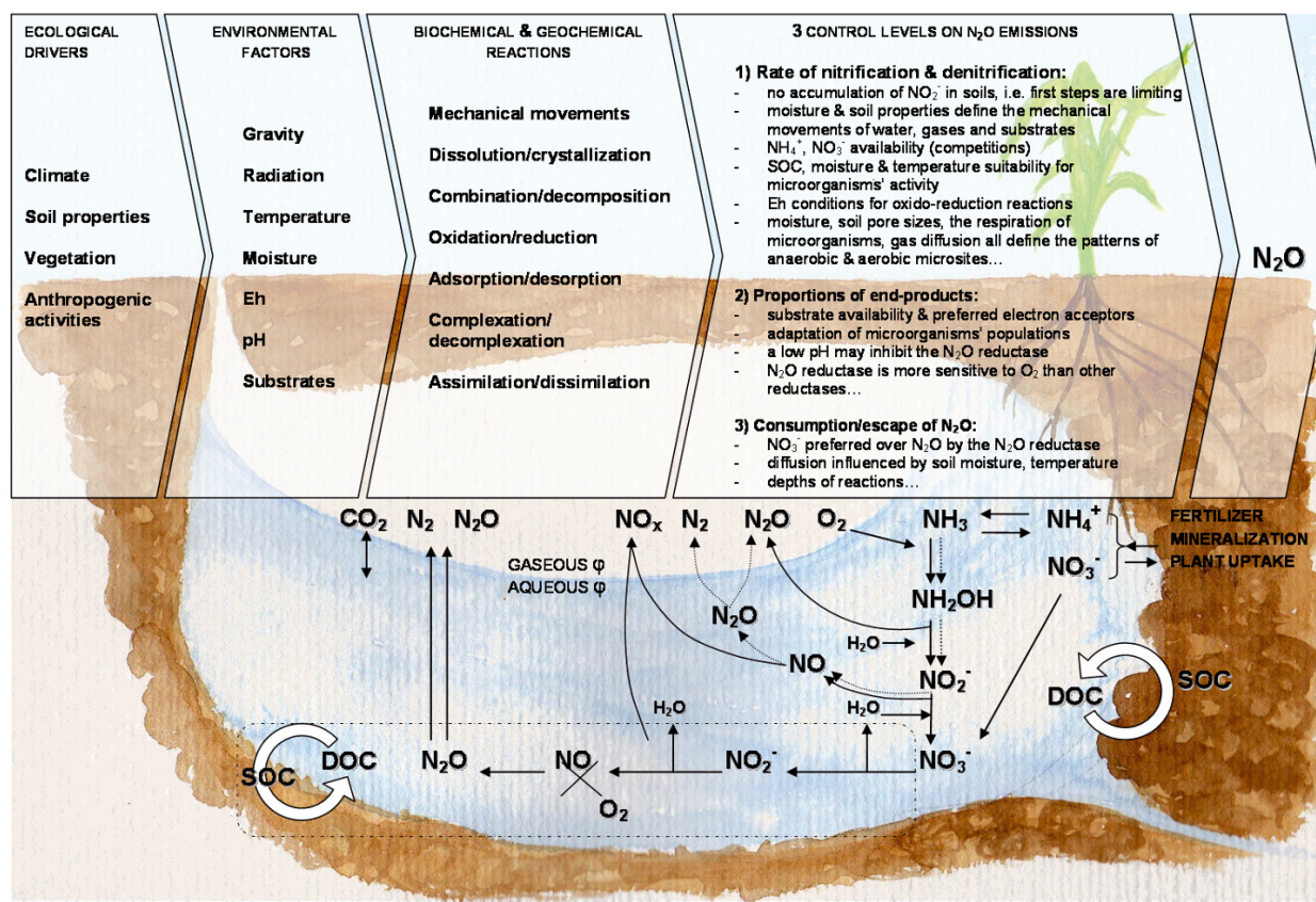
Figure 15. Scheme of the determinism of \text{N}_2\text{O} emissions by soils adapted from Li (2007); Wrage et al. (2005); Farquharson and Baldock (2008). Soil particles, gaseous and aqueous phases ( \phi ) are artificially “well distinguished”. The two extremities of the symbolised pore represent the pore continuum throughout the soil matrix. Reactions take place at the interface of soil particles and aqueous phase where microorganisms and substrates are. Denitrification takes place in the “anaerobic dashed-line rectangle”. Dashed arrows lead to \text{N}_2\text{O} emissions by nitrifier denitrification occurring in low \text{O}_2 conditions, which implies that some \text{NH}_3 oxidisers process the whole reaction chain (Wrage et al., 2001).
