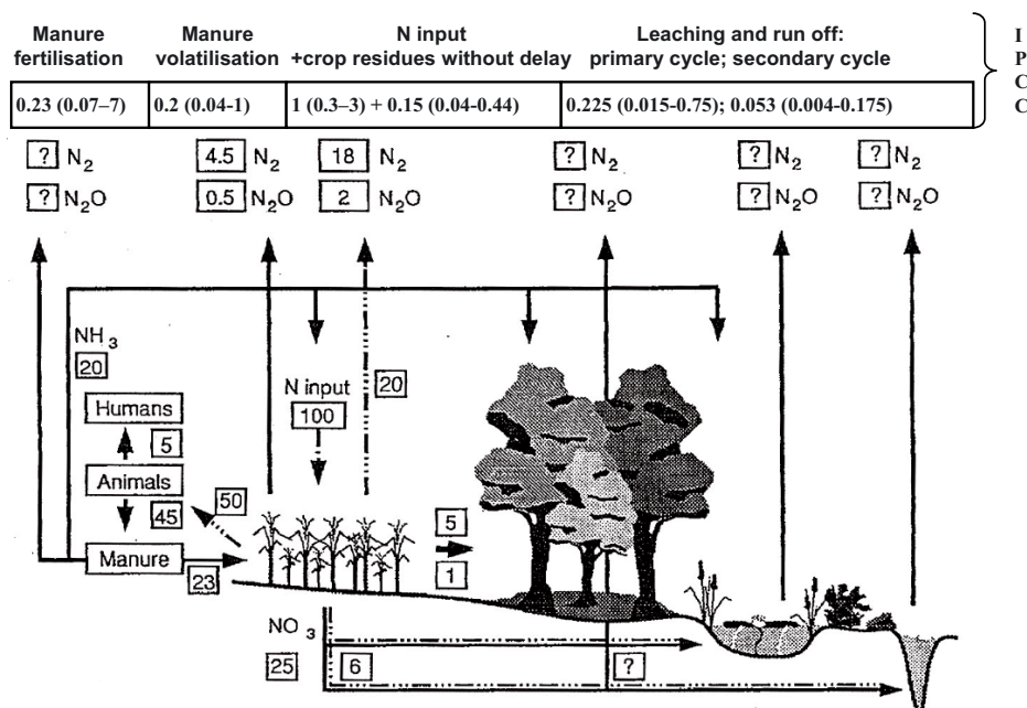
Figure 14. A simplified flow of fertilizer N through the environment (Duxbury and Mosier, 1993) and \text{N}_2\text{O} emissions with ranges into brackets ( \text{N}_2\text{O-Nkg} ) estimated with the IPCC Tier 1 method (IPCC, 2006) considering some US average data on the diverse fractions as given by Duxbury and Mosier (1993).
