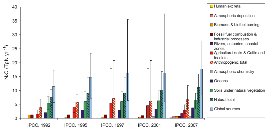
Figure 13. IPCC assessments of total annual \text{N}_2\text{O} emission during the 1990s. Drawn from IPCC data in Mosier et al. 1998 and Denman et al., 2007. Note: for the 1997 assessment 0.9 \text{ Tg yr}^{-1} (\text{Mt yr}^{-1}) of emissions by agricultural soils are subtracted to the total 6.3 \text{ Tg yr}^{-1} (\text{Mt yr}^{-1}) to prevent double counting with part of indirect agricultural emissions already accounted for within emissions by oceans. Emissions from human excreta, rivers and atmospheric deposition can also be partly considered as agricultural indirect emissions.
