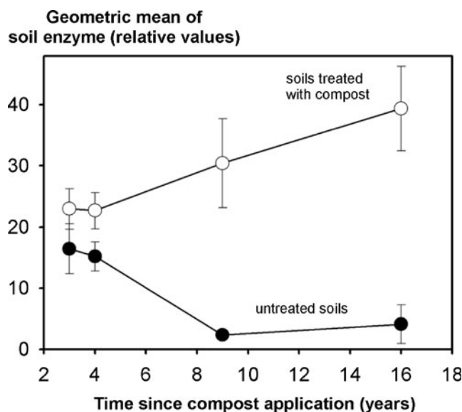
Fig. 2 Geometric mean of assayed soil enzyme for soils which received compost of olive mill pomace for different number of years and for non-compost soils. The geometric mean was higher in the compost-treated soils and differences between treated and untreated increased along the number of years compost was applied
