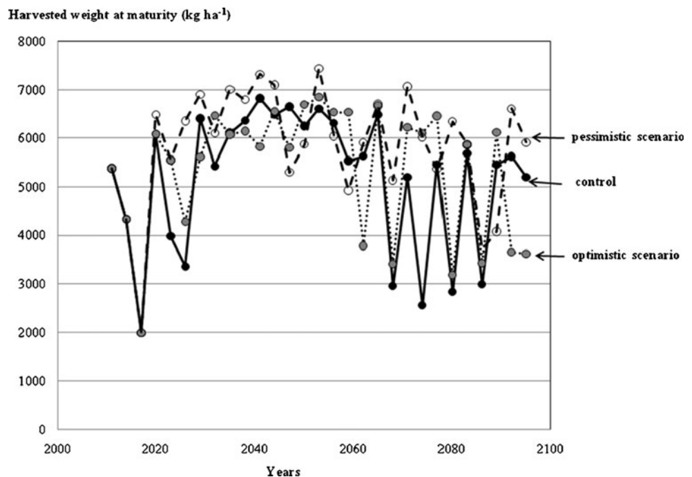
Fig. 3 Simulations of the grain yields of rice from 2011 to 2095 under three climatic conditions. Control no climate change, optimistic scenario a gradual increase in CO 2 up to 750 ppm and a rise in temperature of 0.15°C per decade, pessimistic scenario a gradual increase in CO 2 , a rise in temperature of 0.5°C per decade, and a reduction in rainfall (-0.2 mm day -1 ) from December to February
