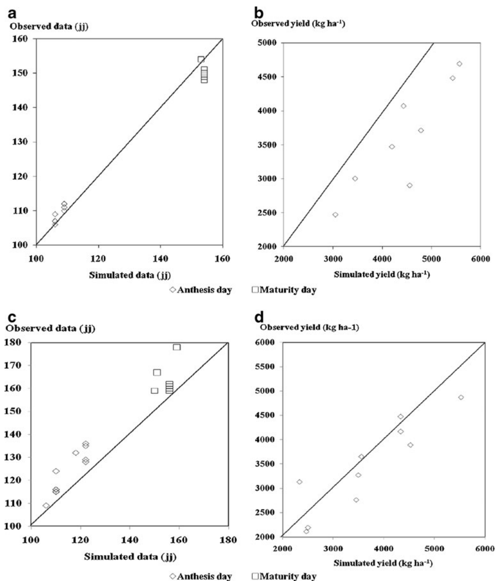
Fig. 2 Simulated and observed data used for calibration, phenology (a), and yield (b) and validation, phenology (c) and yield (d)
