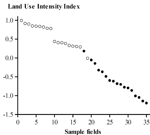
Fig. 1 The land use intensity index for the conventional ( empty circles ) and organic ( black circles ) fields, obtained from the scores of the PCA (see Section 2.3)
