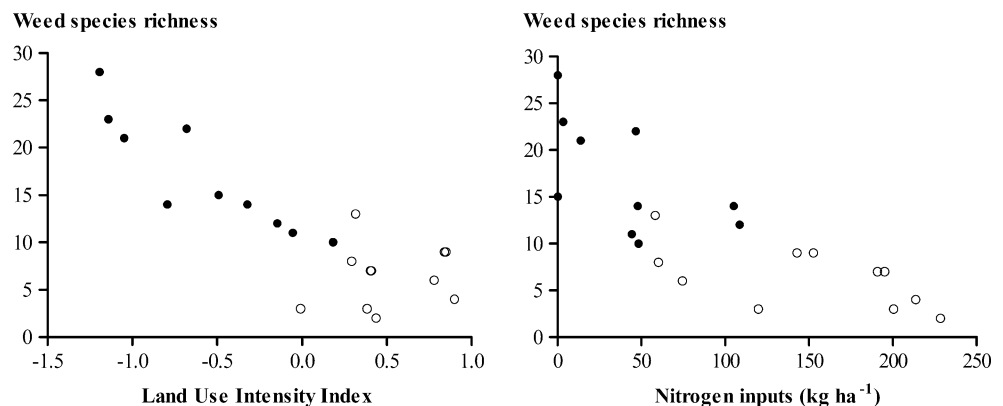
Fig. 2 Weed species richness in relationship to the land use intensity index and nitrogen inputs for the conventional (empty circles) and the organic fields (black circles)
