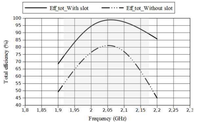
Fig. 4. Comparison of the simulated total efficiency for the system with and without slot.
