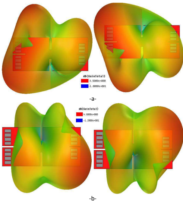
Fig. 9. 3D simulated radiation pattern: (a) left (port 1 excited), right (port 2 excited) at 2.05GHz, (b) left (port 3 excited), right (port 4 excited) at 2.55GHz
