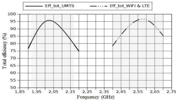
Fig. 8. Simulated total efficiency for the isolated UMTS, WIFI and LTE multi-antenna system.
