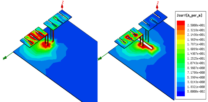
Fig. 3. Surface current distribution for the no-isolated and isolated UMTS multi-antenna system.
