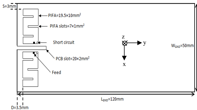
Fig. 1. Top view of the UMTS isolated multi-antenna system.
