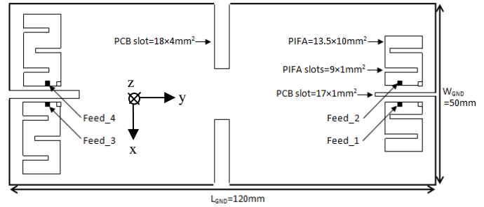
Fig. 6. Top view of the UMTS, WIFI and LTE isolated multi-antenna system.
