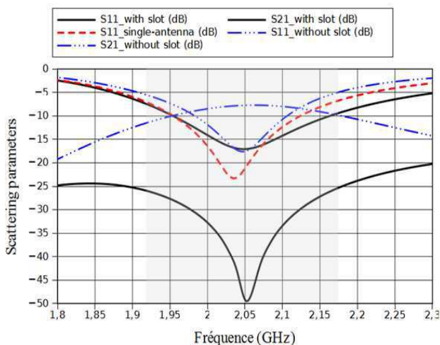
Fig. 2. Simulated scattering parameters results.
