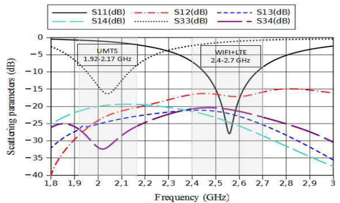
Fig. 7. Simulated scattering parameters results.
