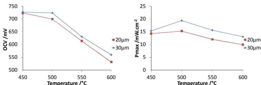
Figure 6. OCV and maximum power density versus temperature for the two investigated electrolyte thickness
