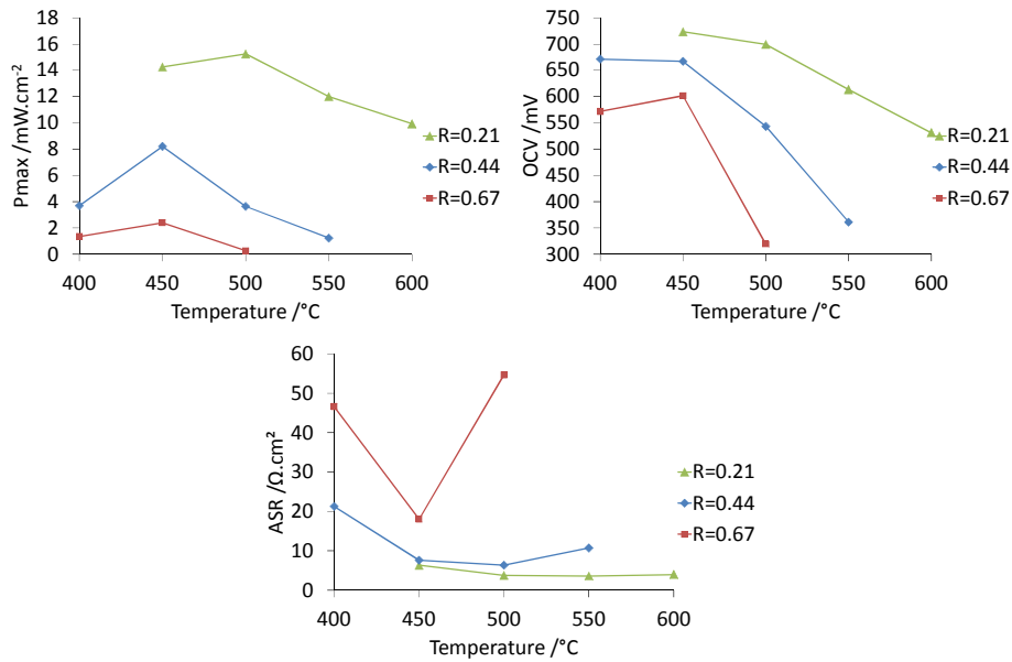
Figure 2. Evolutions of maximum power density, OCV and ASR measured for the three ratios versus temperature
