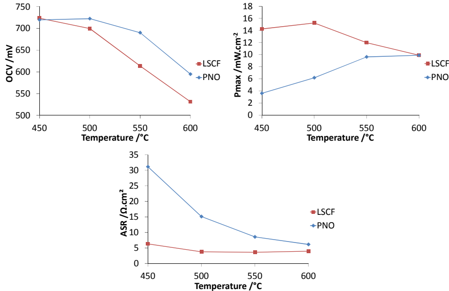
Figure 4. Maximum power density, OCV and ASR versus temperature for the two investigated cathode materials
