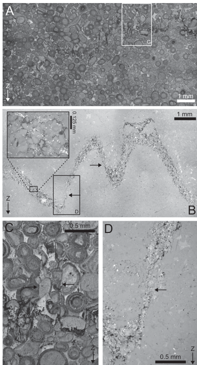
Figure 3. A: Optical photomicrograph map of a sample of O3 containing a thin (50–200 \mu\text{m} ) stylolite. B: Optical photomicrograph map of a sample of D3 containing a thick (1500–3000 \mu\text{m} ) stylolite. Black arrows point to positions where the stylolite is at or close to zero thickness. Inset shows the discontinuous nature of the pressure-solution seams forming the macroscopic stylolite seam. C and D: Optical photomicrographs of a sample of O3 (C) and D3 (D) containing a thin and thick stylolite, respectively. Black arrows point to positions where the stylolite is at or close to zero thickness. Locations of these images are shown on maps in A and B. All photomicrographs are of polished thin sections viewed under reflected light. Z-direction indicates direction of borehole drilling (i.e., vertical and perpendicular to bedding).
