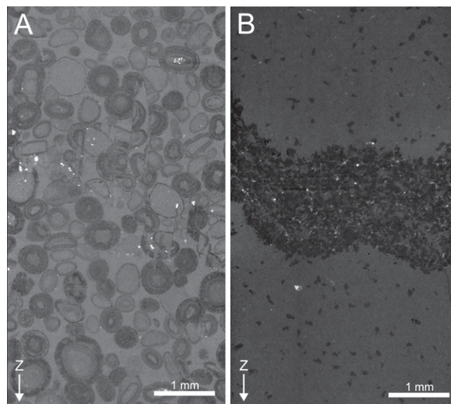
Figure 4. High-resolution (4 \mu\text{m} ) X-ray computed tomographic images of a thin stylolite (50–200 \mu\text{m} ; sample O3) (A) and, a thick stylolite (1500–3000 \mu\text{m} ; sample D3) (B). Dark gray concentric bands within the ooids in A represent bands with a higher porosity (microporosity); light gray is calcite that contains significantly less microporosity. Dark gray minerals in B are quartz grains; light gray is calcite. White dots in A and B are pyrite grains. Z-direction indicates direction of borehole drilling (i.e., vertical and perpendicular to bedding).
