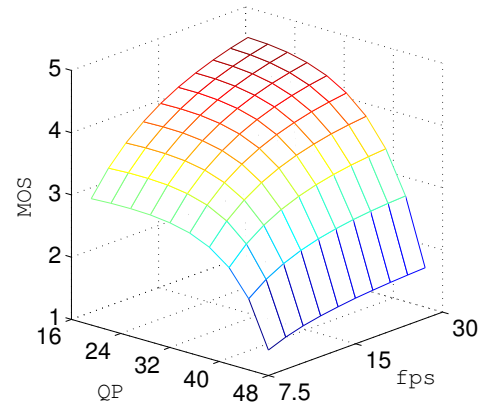
Fig. 3. QoE estimation for SVC videos using PSQA tool.
