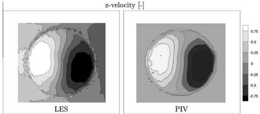
Fig. 8. z-velocity: comparison PIV and LES.
