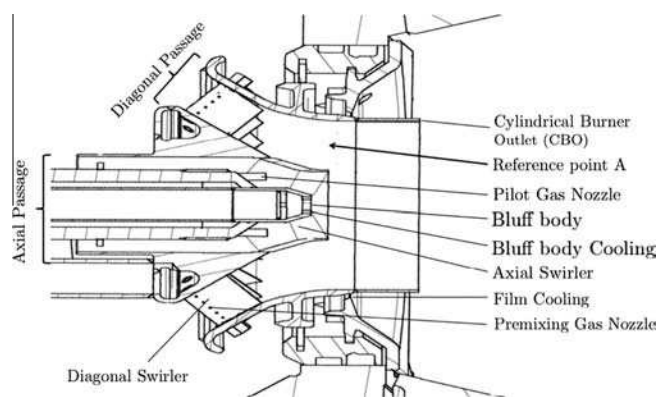
Fig. 1. Burner details and reference point A (proportions changed).
