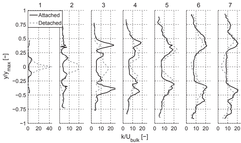
Fig. 21. Turbulent kinetic energy profiles for the Attached and Detached flame (mean fields).
