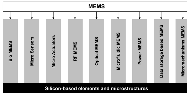
Figure 1: MEMS applications.
