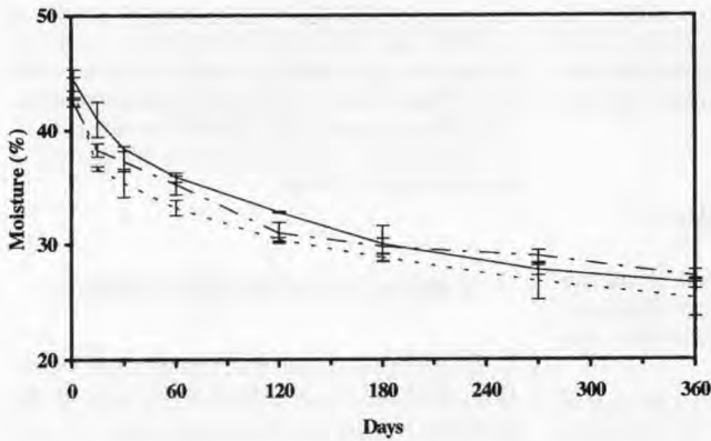
Figure 2. Changes in the moisture content of the 12-h (— low-salted), 24-h (--- medium-salted) and 36-h brined (--- high-salted) cheeses during ripening.
