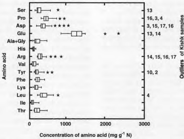
Figure 3. Box plot of concentration of amino acids of the Lebanese Kishk samples. (For sample identification, refer to [48].) The vertical line inside the box represents the median and the vertical ends of the box represent the 1st and 3rd quartiles. Asterisks represent outliers which are further out than 1.5 \times inter-quartile range from the 1st and 3rd quartiles, respectively.
