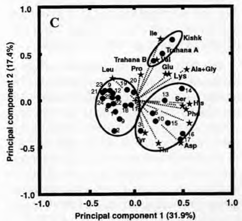
Figure 4. Principal component biplots of amino acids present in the Kishk samples (A), vis-a-vis in skimmed milk powder (SMP) and Burghol (B) and in two Trahana and one Lebanese Kishk products (C). (For sample identification, refer to [48]).
