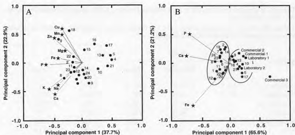
Figure 6. Principal component biplots of mineral contents in the Kishk samples (A), and of P, Ca and Fe of the same samples compared with three commercial and two laboratory-made Kishks (B). (For sample identification, refer to [48]).
