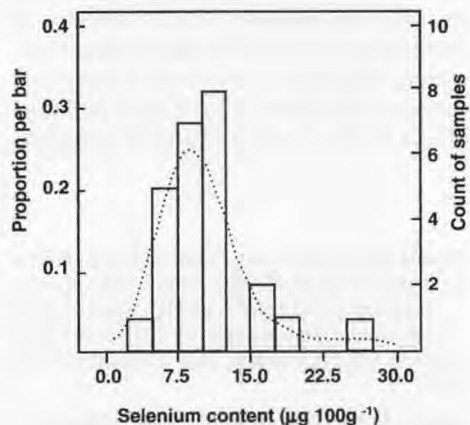
Figure 5. A histogram illustrating the distribution of selenium content in the Kishk samples.
