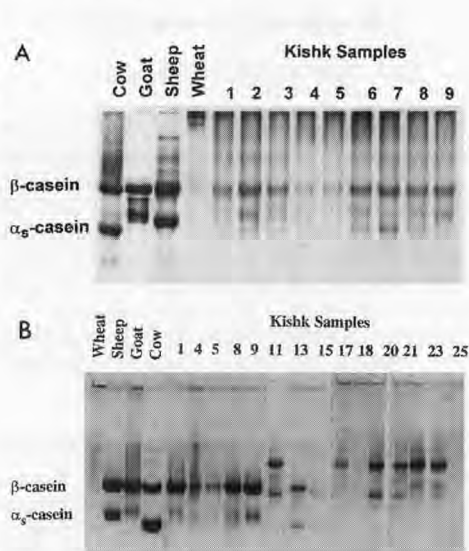
Figure 1. Polyacrylamide gel electrophoresis (PAGE; methods A and B) assay of some Kishk samples. (For sample identification refer to Tamime et al. [46].) A: urea-PAGE (method A); B: discontinuous PAGE (method B). (After Tamime et al. [45].)
