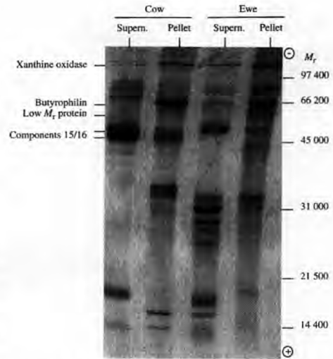
Figure 1. Electrophoresis (15 % [w/v] polyacrylamide, 0.1 % [w/v] sodium dodecyl sulphate, pH 8.8) of supernatants (Supern.) and pellets (Pellet) after ultracentrifugation of the bovine and ovine milk fat globule membranes.
