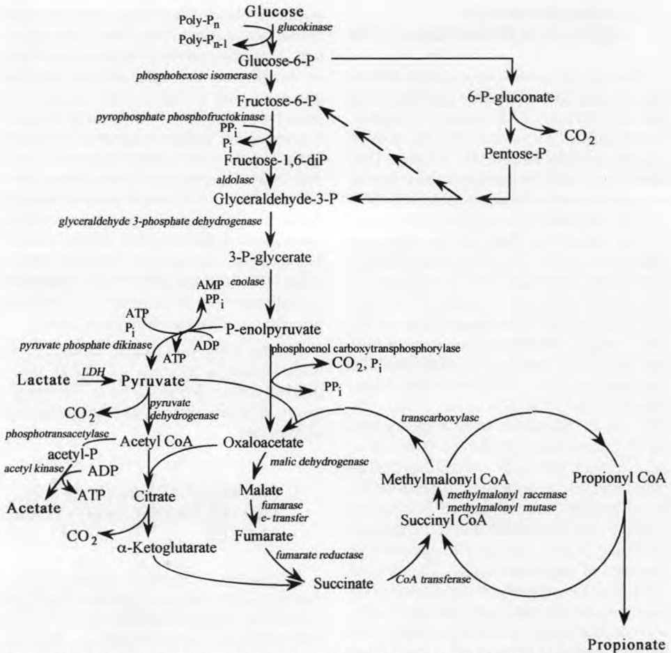
Figure 1. Cycles involved in the propionic acid fermentation (Wood [108]). LDH: lactate dehydrogenase; Poly-P n : polyphosphate; PP i : pyrophosphate. For reasons of clarity, only the pyrophosphate dependent conversion of fructose-6-P to fructose-1,6-diP is shown and ATP generation by the electron transfer system is omitted. All the reactions are directed towards propionate production, even though the reactions are reversible.
