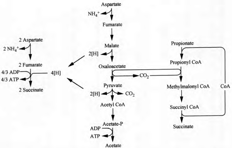
Figure 3. Pathway of aspartate plus propionate fermentation according to Rosner and Schink [75].
