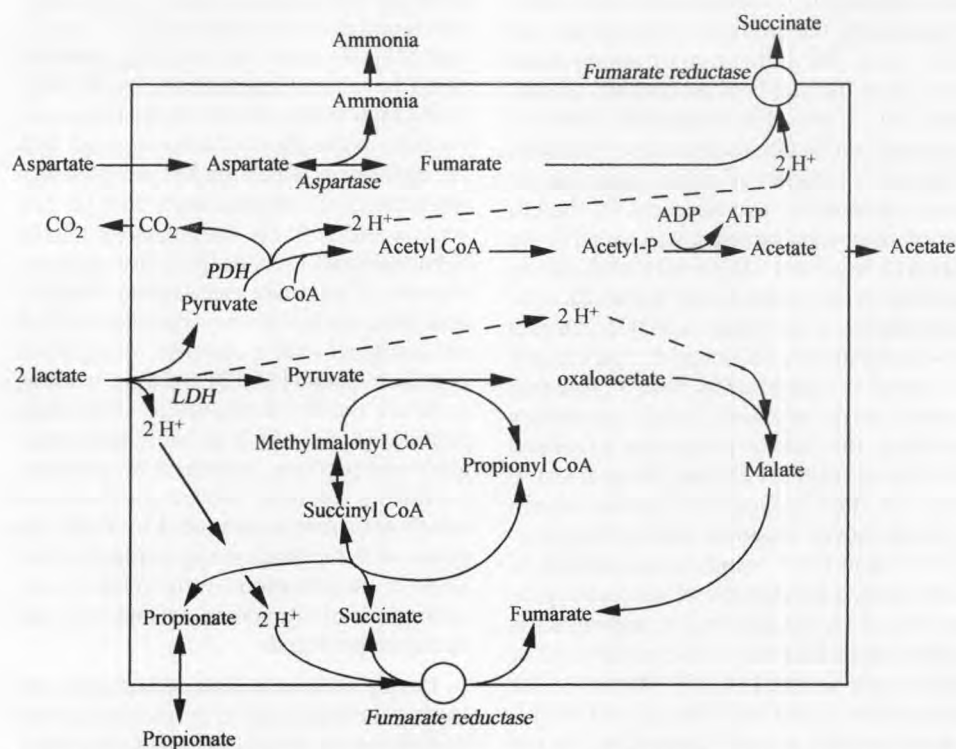
Figure 2. Aspartate and lactate metabolism according to Crow [17]. PDH, pyruvate dehydrogenase. LDH lactate dehydrogenase.
