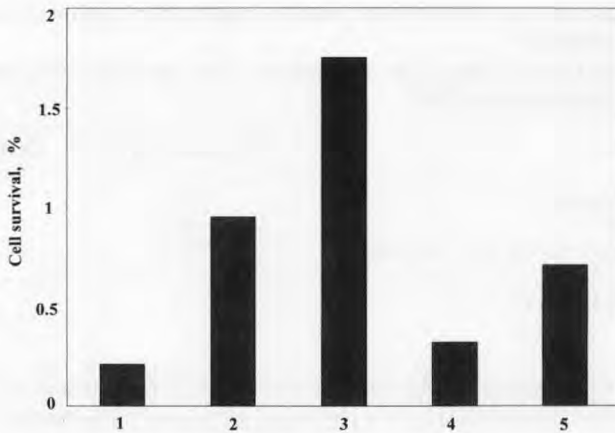
Figure 3. Protective effect of the nucleoprotein complex (NPC) in UV-inactivated E. coli AB1157 after enzymatic treatment. 1. Control (without protective factor). 2. Preincubation with nucleoprotein complex (NPC). 3. NPC treated with pronase. 4. NPC treated with DNase. 5. NPC treated with RNase.
