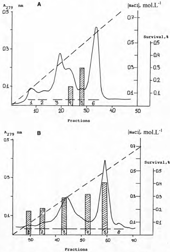
Figure 2. Separation of AF1-2 and AF2-2 fractions by anion-exchange chromatography on DEAE-sepharose. A. Separation of active proteins of AF1-2. B. Separation of active proteins of AF2-2. Continuous line—boundaries of subfractions; subfractions are numbered; shade columns show cell viability in % in the presence of respective subfractions.
