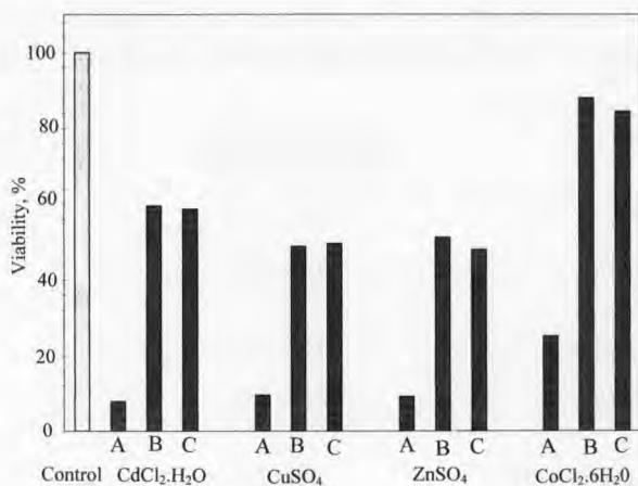
Figure 1. Protective and reactivative action of the cell-free extract (CFE) of P. shermanii VKM-103 on E. coli AB1157 inactivated by exposure to the salts of heavy metals. A. Without CFE. B. With preincubation. C. With postincubation.
