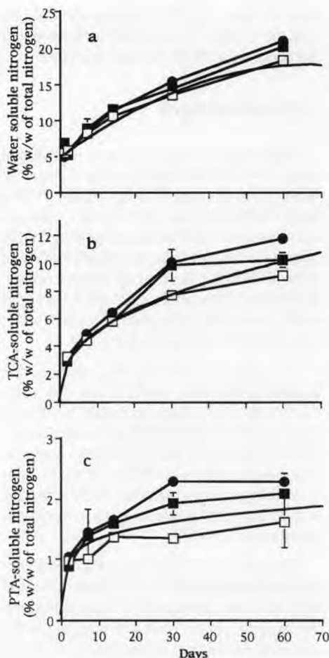
Figure 1. Production of water-soluble nitrogen (a), TCA-soluble nitrogen (b) and PTA-soluble nitrogen (c) during ripening. NL (—); L0 (□); L1 (■); L2 (●) cheeses. The response for the control cheeses (NL) was represented by the best fitted curve for water-soluble nitrogen ( r = 0.996 ), TCA-soluble nitrogen ( r = 0.998 ); PTA-soluble nitrogen ( r = 0.957 ).
