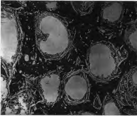
Figure 4. Microstructure of HL cheeses after one week of ripening. Bar represents 2 \mu\text{m} .
