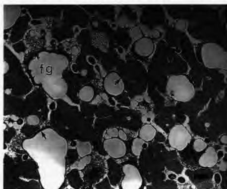
Figure 3. Microstructure of NL cheeses after one week of ripening. Bar represents 2 \mu m. fg: fat globule; cm: casein matrix; arrow: fat globule membrane.
