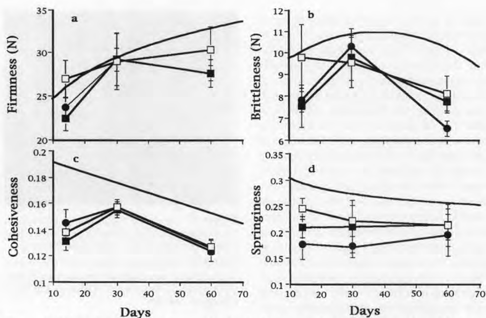
Figure 9. Effect of the ripening time on the rheological properties of NL cheeses (—); L0 cheeses (□); L1 cheeses (■); L2 cheeses (●). The response of the control cheeses (NL) were modeled with the best-fitted curve for firmness ( r = 0.998 ); brittleness ( r = 1.0 ); cohesiveness ( r = 0.992 ); springiness ( r = 0.994 ).
