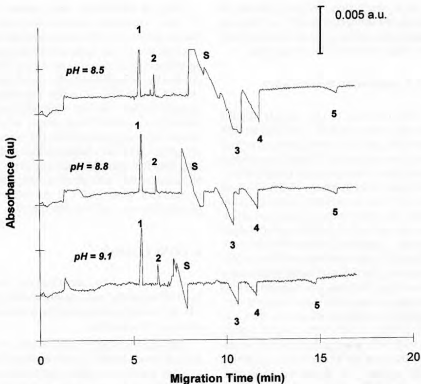
Figure 1. Electropherograms of sweet whey anions with BGE at various pHs: pH 8.5 (electrolyte 1); pH 8.8 (electrolyte 4); pH 9.1 (electrolyte 5). Samples: 25-fold water dilution of 60 g/L whey solution. Standard CE (see Materials and methods ). Electrolyte compositions ( table I ). Peak identification as follows: 1, chloride; 2, sulfate; 3, citrate; 4, phosphate; 5, carbonate; S, system peak.
