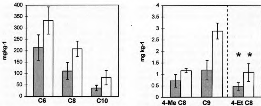
Figure 1. Specific goat aroma compounds in A (■) and O (□) cheeses at day 13 ( n = 4 ). Levels in \text{mg kg}^{-1} ; (*) Values \times 10 on the graph. Bars: standard deviation.
