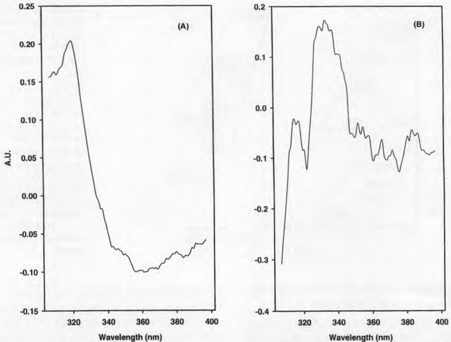
Fig 4. Spectral patterns corresponding to the principal component 1 (A) and 2 (B). Fluorescence emission spectra of tryptophans.
