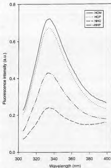
Fig 2. Tryptophan fluorescence spectra of the creams prepared from NHO, NHP, HOM and HOP milk samples. See Materials and methods for details.
