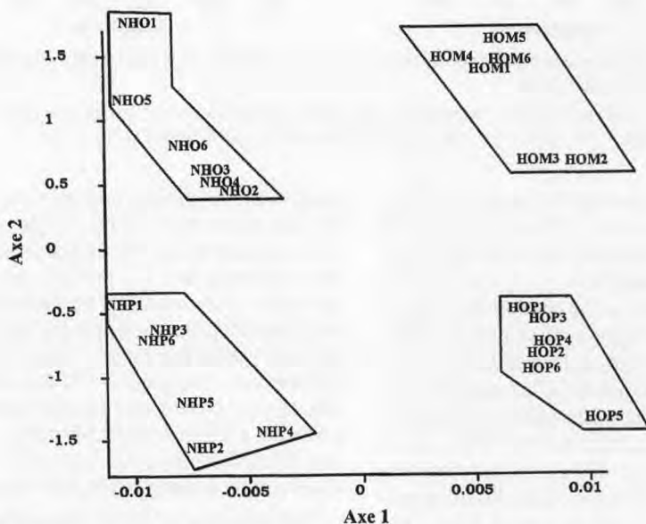
Fig 6. PCA similarity map defined by the principal components 1 and 2 for the data table including tryptophan emission, retinol excitation and ANS excitation spectra. Each label corresponds to a spectrum. See Materials and methods for details.
