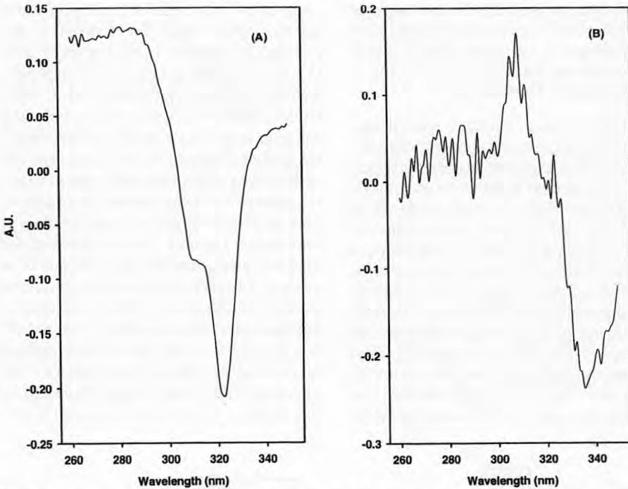
Fig 5. Spectral patterns corresponding to the principal component 1 (A) and 2 (B). Fluorescence excitation spectra of vitamin A.
