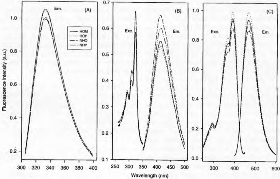
Fig 1. Fluorescence spectra of NHO, NHP, HOM and HOP milk samples. A. Tryptophan emission spectra. B. Excitation and emission spectra of vitamin A. C. Excitation and emission spectra of ANS. Exc, excitation spectrum; Em, emission spectrum. See Materials and methods for details.
