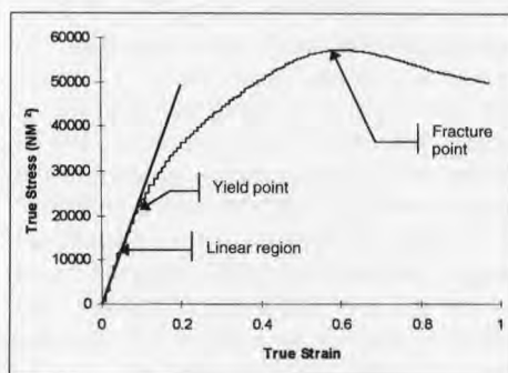
Fig 1. Typical stress strain curve for Cheddar cheese.
