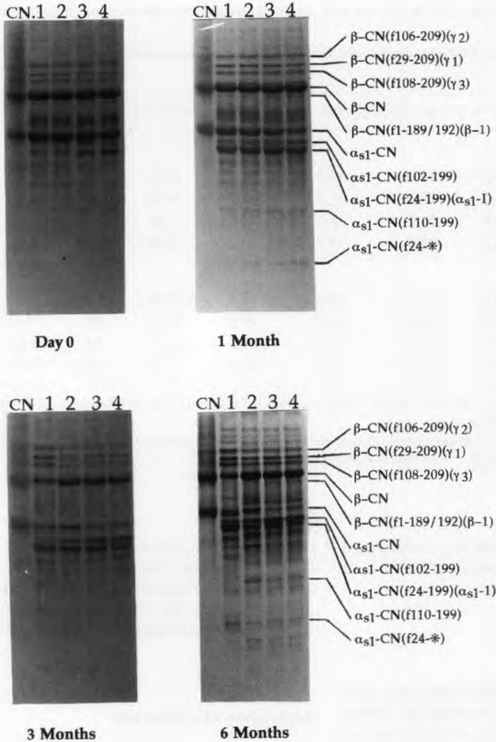
Fig 2. Urea-polyacrylamide gel electrophoretograms of bovine sodium caseinate (CN) and whole Cheddar cheese samples from trial 1 at different stages of ripening. Cheeses manufactured under controlled microbiological conditions using glucono- \delta -lactone (GDL) (lane 1), GDL/Lb adjunct (lane 2), starter (lane 3) or starter/Lb adjunct (lane 4). * Undetermined C-terminus.
