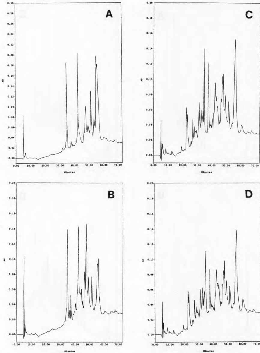
Fig 6. Reverse-phase HPLC chromatograms of the water-soluble/700 mL/L ethanol-insoluble fraction from 6-month-old Cheddar cheeses (trial 1) manufactured under controlled microbiological conditions, with or without adjunct lactobacilli by chemical ( A , glucono- \delta -lactone [GDL]; B , GDL/Lb adjunct) or biological ( C , starter; D , starter/Lb adjunct) acidification.
