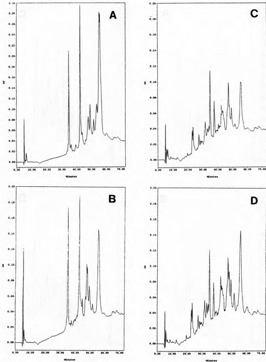
Fig 5. Reverse-phase HPLC chromatograms of the water-soluble/700 mL/L ethanol-insoluble fraction from 3-month-old Cheddar cheeses (trial 1) manufactured under controlled microbiological conditions, with or without adjunct lactobacilli by chemical (A, glucono- \delta -lactone [GDL]; B, GDL/Lb adjunct) or biological (C, starter; D, starter/Lb adjunct) acidification.
