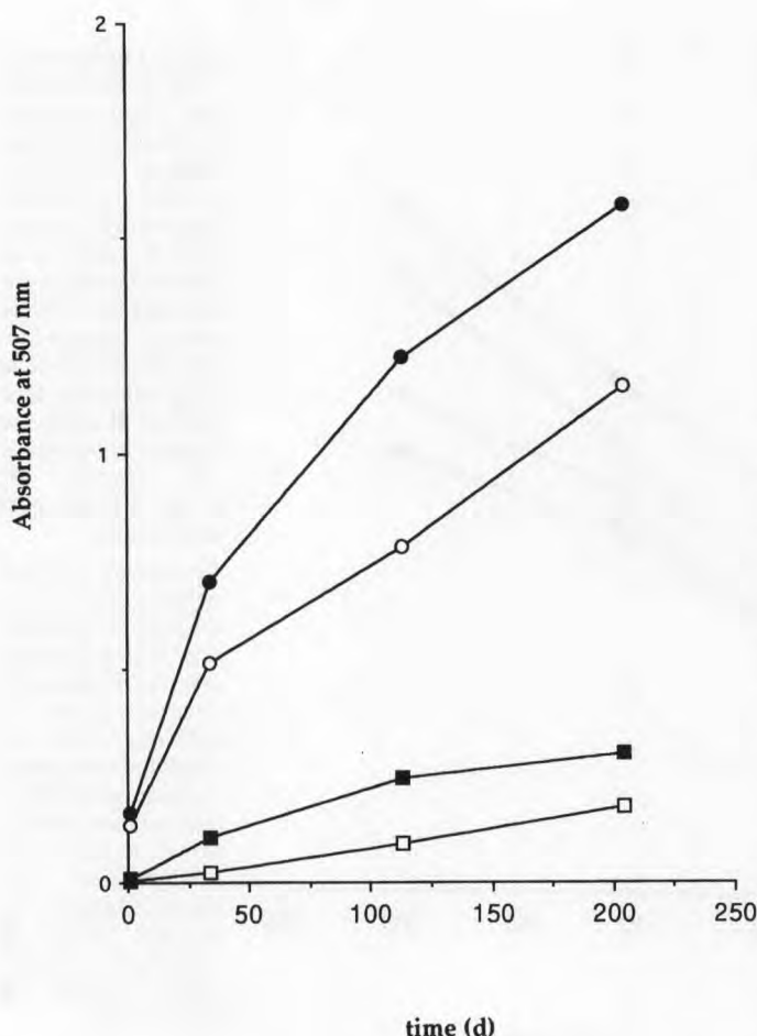
Fig 4. Formation of total free amino acids in Cheddar cheeses (trial 1) manufactured under controlled microbiological conditions, with or without adjunct lactobacilli, by chemical (□, glucono- \delta -lactone [GDL]; ■, GDL/Lb adjunct) or biological (○, starter; ●, starter/Lb adjunct) acidification.
