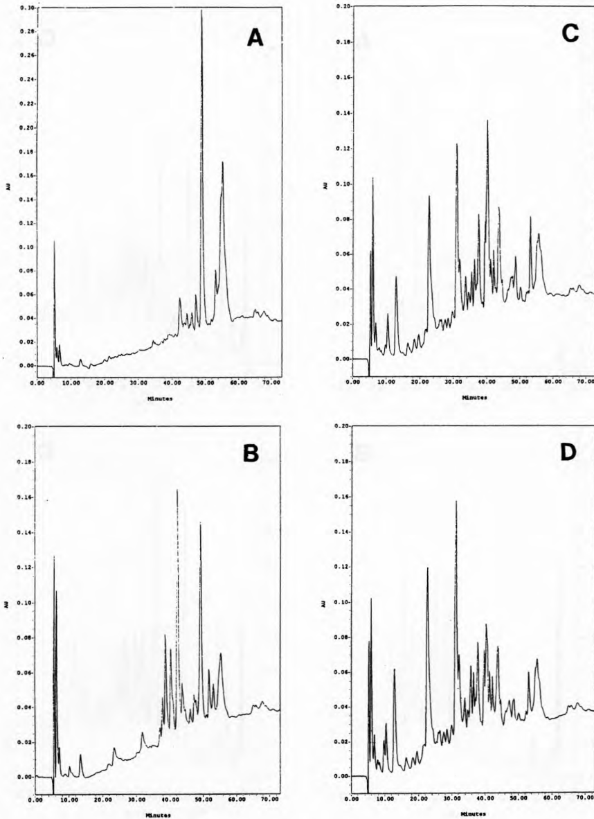
Fig 7. Reverse-phase HPLC chromatograms of the water-soluble/700 mL/L ethanol-soluble fraction from 3-month-old Cheddar cheeses (trial 1) manufactured under controlled microbiological conditions, with or without adjunct lactobacilli by chemical (A, glucono- \delta -lactone [GDL]; B, GDL/Lb adjunct) or biological (C, starter; D, starter/Lb adjunct) acidification.
