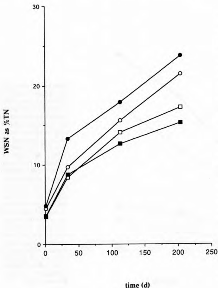
Fig 3. Formation of water-soluble nitrogen, expressed as a percentage of total nitrogen (WSN as % of TN) in Cheddar cheeses (trial 1) manufactured under controlled microbiological conditions, with or without adjunct lactobacilli, by chemical (□, glucono- \delta -lactone [GDL]; ■, GDL/Lb adjunct) or biological (○, starter; ●, starter/Lb adjunct) acidification.
