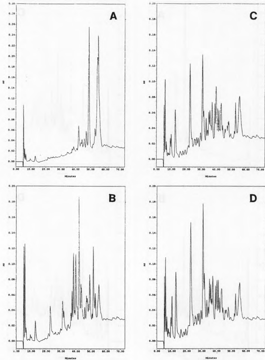
Fig 8. Reverse-phase HPLC chromatograms of the water-soluble/700 mL/L ethanol-soluble fraction from 6-month-old Cheddar cheeses (trial 1) manufactured under controlled microbiological conditions, with or without adjunct lactobacilli by chemical ( A , glucono- \delta -lactone [GDL]; B , GDL/Lb adjunct) or biological ( C , starter; D , starter/Lb adjunct) acidification.
