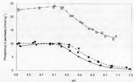
Fig 3. Solubilization of phosphorus from native phosphocaseinate suspensions dissolved in water, 0.1 \text{ mol L}^{-1} NaCl and UF with the decrease of pH at 20^\circ\text{C} . Concentrations of phosphorus in permeates obtained by ultrafiltration on Centriflo CF25 are presented. The pH values were obtained after the addition of GDL during 15h at 20^\circ\text{C} . Two replicates for each medium are presented. Same symbols as in the legend to figure 1.
