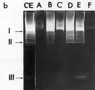
Fig 6. Elution profile (a) of P70 extract on gel permeation chromatography (Superose 12) (50 mmol/l potassium phosphate buffer, pH 5.8 containing 50 mmol/l KCl) and (b) renaturing SDS-PAGE profiles of the fractions obtained: lanes 1: CE; 2: A; 3: B; 4: C; 5: D; 6: E; 7: F (Renaturation buffer: 0.1 mol/l potassium phosphate buffer pH 5.8 - Triton X-100); (Lytic activities: I: 120 kDa; II: 81 to 118 kDa; III: 34 kDa).
