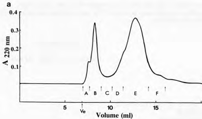
Fig 6. Elution profile (a) of P70 extract on gel permeation chromatography (Superose 12) (50 mmol/l potassium phosphate buffer, pH 5.8 containing 50 mmol/l KCl) and (b) renaturing SDS-PAGE profiles of the fractions obtained: lanes 1: CE; 2: A; 3: B; 4: C; 5: D; 6: E; 7: F (Renaturation buffer: 0.1 mol/l potassium phosphate buffer pH 5.8 - Triton X-100); (Lytic activities: I: 120 kDa; II: 81 to 118 kDa; III: 34 kDa).
