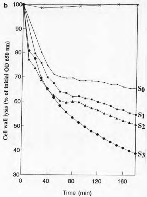
Fig 4. (a) Cell wall lysis in 0.05 mol/l KCl (1.46 mg dry weight isolated cell walls/ml) (●) and concomitant evolution of the protein content (■) of supernatants (S0, S1, S2, S3) obtained by centrifugation at 0, 40, 90 and 160 min of lysis. (b) These 4 supernatants (2 ml), concentrated by ultrafiltration to 100 µl, were able to hydrolyse heat-isolated cell walls (10 min at 100°C), suspended in 0.1 mol/l potassium phosphate buffer (pH 5.8; 40°C) at 0.6 mg dry weight isolated cell walls/ml. (c) SDS-PAGE of the total cell wall proteins before lysis (lane 1), of the supernatant S2 (lane 2), S2 after concentration by centricon C10 (lane 3), S2 after concentration by centricon C30 (lane 4). The gel was stained using silver nitrate.
