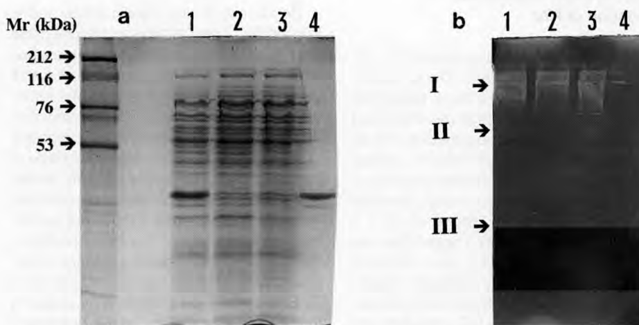
Fig 5. (a) Protein profiles and (b) profiles after renaturing SDS-PAGE of the following extracts: lane 1: CE; lane 2: pellet sulfate ammonium precipitation of CE at 70% (P70); lane 3: supernatant of CE sulfate ammonium precipitation at 70% (S70); lane 4: pellet sulfate ammonium precipitation of CE at 50% (P50). (Renaturation buffer: 0.1 mol/l potassium phosphate, pH 5.8 with 1 % (w/v) Triton X-100; 40°C). (Lytic activities: I: 120 kDa; II: 81 to 118 kDa; III: 34 kDa).
