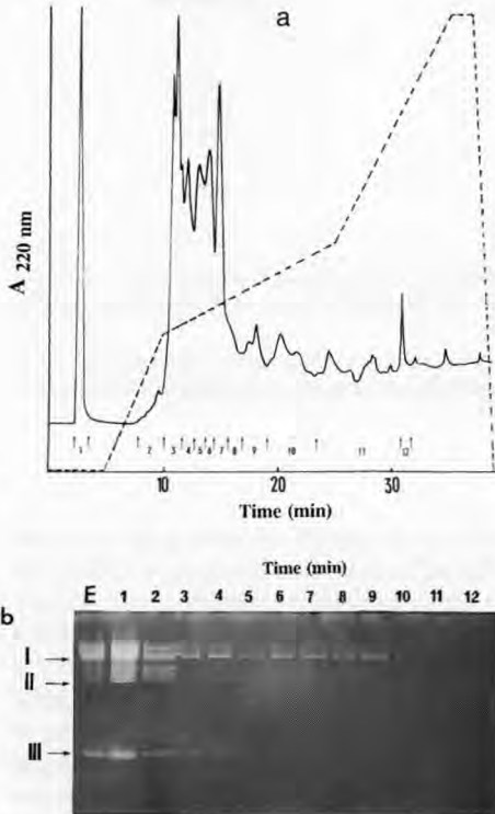
Fig 7. Elution profile of the fraction E, obtained in figure 6 by gel permeation, on (a) anion exchanger chromatography (Mono Q) and (b) renaturing SDS-PAGE profiles of the fractions obtained: lane 1: E fraction; lanes 2 to 13: the 12 pooled fractions obtained by chromatography, called 1 to 12. (Renaturation buffer: 0.1 mol/l potassium phosphate buffer pH 5.8 - Triton X-100); (Lytic activities: I: 120 kDa; II: 81 to 118 kDa; III: 34 kDa).
