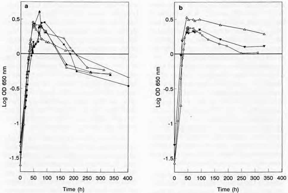
Fig 1. Comparison of the growth curves ( \log OD_{650} ) in YEL medium at 30°C, of (a) dairy propionibacteria strains highly prone to autolysis in potassium phosphate buffer (cluster A, strains: CNRZ 725, ■; CNRZ 727, +; TL 12, \Delta ; P, □; T, \blacktriangle ) and (b) strains more resistant to autolysis (cluster B, strains: CNRZ 277, □; M, \Delta ; N, \blacktriangledown ).
