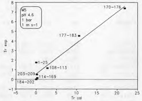
Fig 5. Experimental transmission, Tr_{exp} versus the predicted transmission calculated according to eq (7); Tr_{cal} , peptides; M5, membrane (calculated without taking into account \beta CN 49–97 and \beta CN 100–105).
