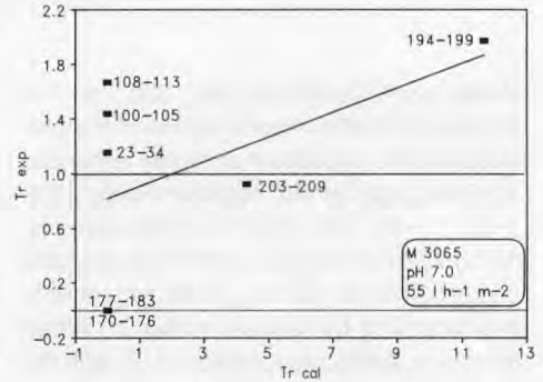
Fig 6. Experimental transmission Tr_{exp} versus the predicted transmission calculated according to eq (7); Tr_{cal} , peptides; 3065 membrane.
