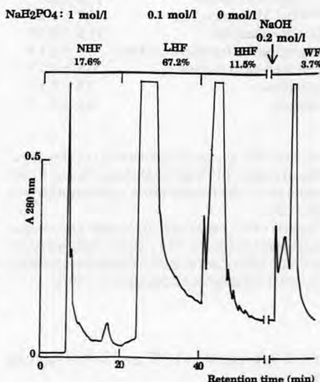
Fig 1. Fractionation of proteose-peptone by semi-preparative hydrophobic interaction FPLC in a TSK-Phenyl 5PW column (method adapted from Girardet et al , 1991). Nitrogen content of each collected fraction was determined by the Kjeldahl method. NHF, non-hydrophobic fraction; LHF, low hydrophobic fraction; HHF, high hydrophobic fraction; WF, wash fraction.
