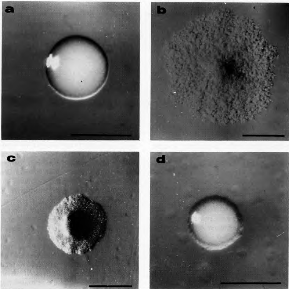
Fig 5. Variant colonies of S thermophilus CNRZ368 on TPPY agar medium. (a): 'opaque'. (b): 'diffuse'. (c): 'ring'. (d) : 'edged'. Colonies were grown for 24 h at 42 °C in aerobic conditions. Bars, 1 mm.
