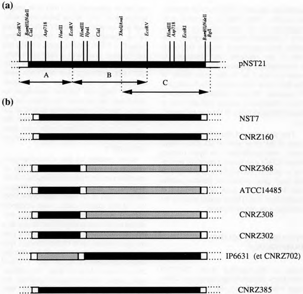
Fig 4. Map of the varA locus in 9 strains of S. thermophilus .
