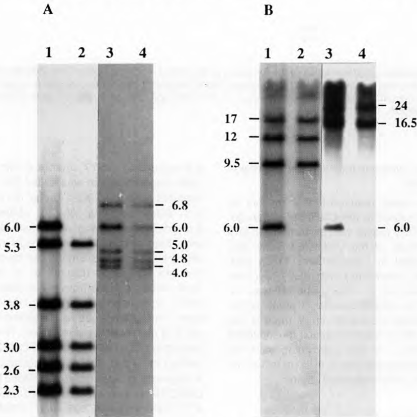
Fig 2. Hybridization patterns of strains CNRZ368 and B210. Fragment sizes are indicated in kilobases. A. Hind III digests. B. Apal digests. Lane 1: CNRZ368 strain hybridized with I41. Lane 2: strain B210 hybridized with I41. Lane 3: CNRZ368 strain hybridized with I43.1. Lane 4: B210 strain hybridized with I43.1.
