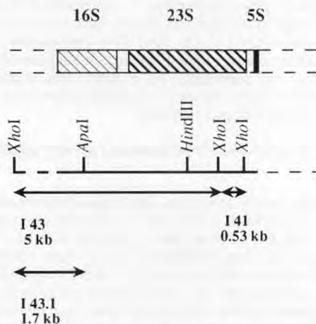
Fig 1. Location of the probes and restriction sites used in this study towards the rrn locus map.
