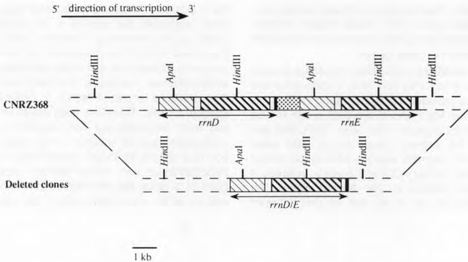
Fig 3. Schematic representation of the formation of the hybrid rrn locus. Dotted lines indicate extra-peronic sequences. Upstream and downstream Hind III fragments remain unchanged in sizes, whereas the internal Hind III fragment disappears. ▨: 16S gene. ▩: 23S gene. ■: 5S gene. ▤: interperonic region.
