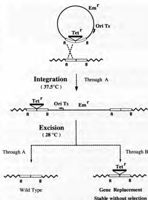
Fig 4. General strategy for replacement recombination: the pG + host plasmid carries a chromosomal DNA fragment (white box) interrupted by a marker (here represented by Tet r ). The initial recombination event occurs by SCO integration (shown here through region A) when liquid cultures are maintained overnight at 37.5°C with selection for the plasmid antibiotic marker (Em r ). Cultures are then diluted and shifted to 28°C. At this temperature, replication of the integrated pG + host (Ori Ts) is activated, and recombination between duplicated sequences is stimulated; this recombination event leads to plasmid excision. Plasmid excision through A restores the parental chromosomal structure, while excision through B produces a gene replacement event. If the initial integration had occurred at B, excision at A would result in gene replacement. Cultures are plated at 37°C, with or without selection for the replacing fragment (Tet r ). If no selection is applied, screening for gene replacement can be performed (we found between 1–40% gene replacement without selection at this step). Symbols: black line, plasmid backbone; wavy line, chromosome; white boxes, regions of homologous chromosomal fragment between the plasmid and the chromosome; hatched box, Em r marker; black box, Tet r marker; Ori Ts, pG + host replication origin.
