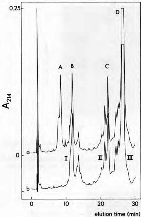
Fig 1. Separation of whole caprine casein by RP-HPLC (Vydac C4 column). Effect of DTT treatment: 10 mmol/l DTT-treated casein (a), unreduced casein (b). Amount of protein injected: 70 \mu g.
