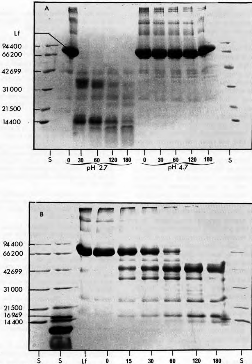
Fig 5. SDS-PAGE of lactoferrin hydrolyzed with rennet for indicated time (min). S = molecular weight standard. Lf = lactoferrin; 4A: pH 2.7 or 4.7, E/S = 1/2500, T = 37 °C. 4B: pH 2.7, E/S = 1/250000, T = 37 °C.
