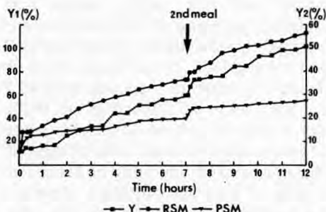
Fig 2. Cumulative amount of immunoreactive \beta -lactoglobulin leaving the abomasum for the three diets in percentage of ingested \beta -lactoglobulin with the first meal (Y1) or in percentage of ingested \beta -lactoglobulin with the 2 meals (Y2).
