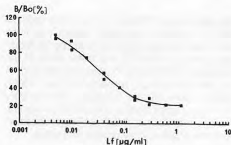
Fig 1. Standard inhibition curves for \beta -lactoglobulin and lactoferrin in ELISA. B/B_0 \cdot 100 = F([\text{BLg or Lf}] ). Courbes étalon des dosages ELISA. B/B_0 \cdot 100 = F([\text{BLg ou Lf}] .
