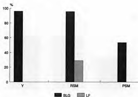
Fig 3. Cumulative amount of immunoreactive \beta -lactoglobulin or lactoferrin emptied during the first 7 h in relation to the emptied fresh matter.
