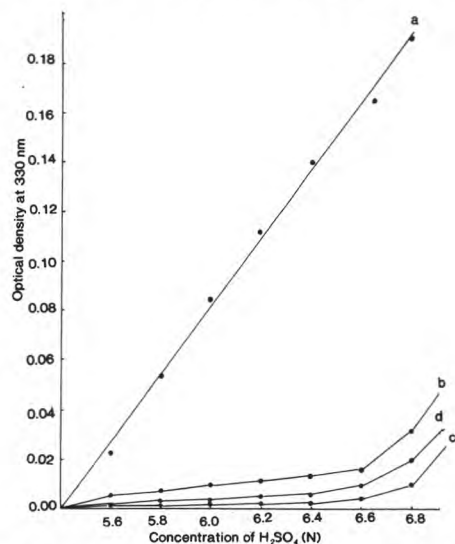
Fig 2. Effect of strength of H_2SO_4 on the colour development of lactulose and other aldoses. a: lactulose (0.016%), b: lactose (1.0%), c: glucose (1.0%), d: galactose (1.0%).
