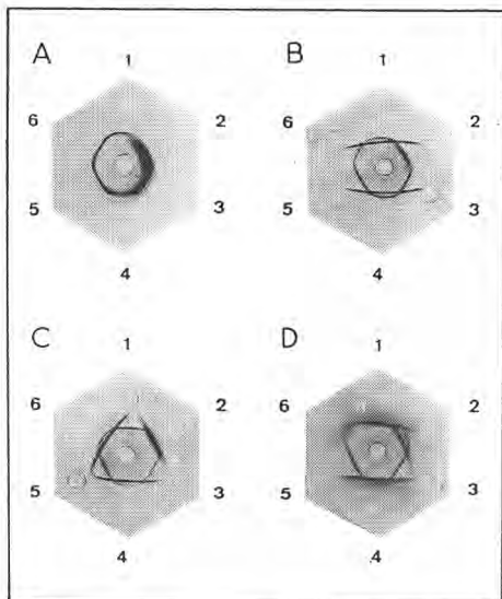
Fig 4. Immunodouble diffusion patterns demonstrating the presence of a contaminant protein in antigenic Plg preparation ( A, B ), in dialysed milk ( C ) and in Plm ( D ). Center wells contain anti-Plg serum; A 1-6: dilution 1/1 to 1/32 of blood Plg 8.5 mg.ml -1 ; B 1,4: Plg (1 mg.ml -1 ); 2,5: immunoglobulin (1 and 0.5 mg.ml -1 ); 3,6: dilution 1/2, 1/4 of dialysed milk; C 1,3,5: dilutions 1/1, 1/2 and 1/4 of dialysed milk; 2,4,6: blood Plg (1, 0.5 and 0.25 mg.ml -1 ); D 1,4: blood Plg (0.5 mg.ml -1 ); 2: Plm; 3,5: immunoglobulins (0.5 mg.ml -1 ).
