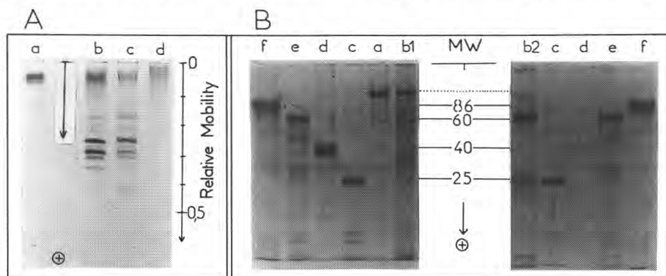
Fig 3. Electrophoretic study of blood enzyme. A PAGE pattern of blood Plg (a), of activated Plg (b, c) and of UK (d). B SDS-PAGE pattern of blood Plg (a), of little activated Plg (b 1 ) and of total activated Plg (b 2 ). Standard Proteins: chymotrypsinogen (c), aldolase (d), catalase (e) and bovine transferrin (f). Molecular weights in kDa.
