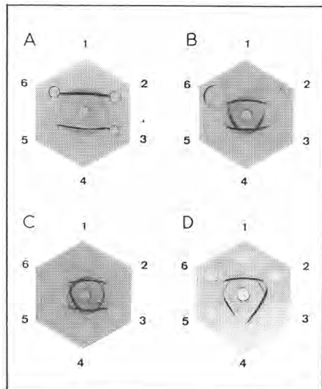
Fig 6. Immunodouble diffusion patterns resulting from the interaction of anti-Plg serum (center wells) and the different MAP preparations obtained from FZ by chromatography on immunoabsorbant (A, B, C) and from whole casein by chromatography on Lysine-Sepharose (D). A : 1,4 : Plg ( 0.5 \text{ mg}\cdot\text{ml}^{-1} ); 2,5: MAP preparation no 1 diluted 1/1 and 1/2; 3,6: MAP preparation no 2 diluted 1/2 and 1/1; B : 1,4 Plg ( 0.5 \text{ mg}\cdot\text{ml}^{-1} ); 2,6: MAP preparation no 2, dilution 1/1; 3 : immunoglobulin ( 0.25 \text{ mg}\cdot\text{ml}^{-1} ); 5 : UK-activated Plg; C : B with MAP preparation no 3, dilution 1/1; D : 1,3 : Plg ( 0.5 \text{ mg}\cdot\text{ml}^{-1} ); 2,6 MAP; 5 : immunoglobulins ( 0.5 \text{ mg}\cdot\text{ml}^{-1} ).
