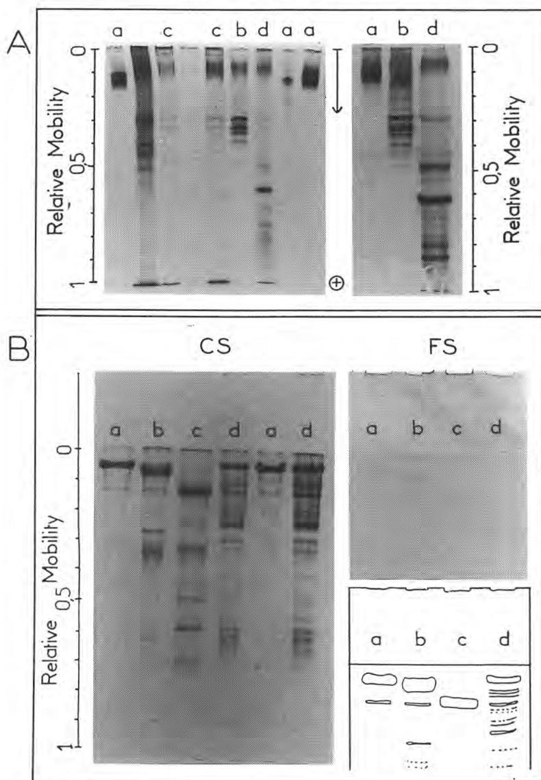
Fig 5. Electrophoretic study of milk enzyme. A : Comparative PAGE patterns of blood Plg (a), of UK-activated Plg (b), of MAP obtained from FZ by affinity chromatographies on Lysine-Sepharose (c) and on immunoabsorbant (d). B : Comparative SDS-PAGE patterns with Coomassie (CS) or Fuchsin (FS) staining of blood Plg (a), of MAP obtained from casein by chromatography on Lysine-Sepharose (b), of MAP obtained from FZ by chromatography on immunoabsorbant (c) and of UK-activated Plg (d).
