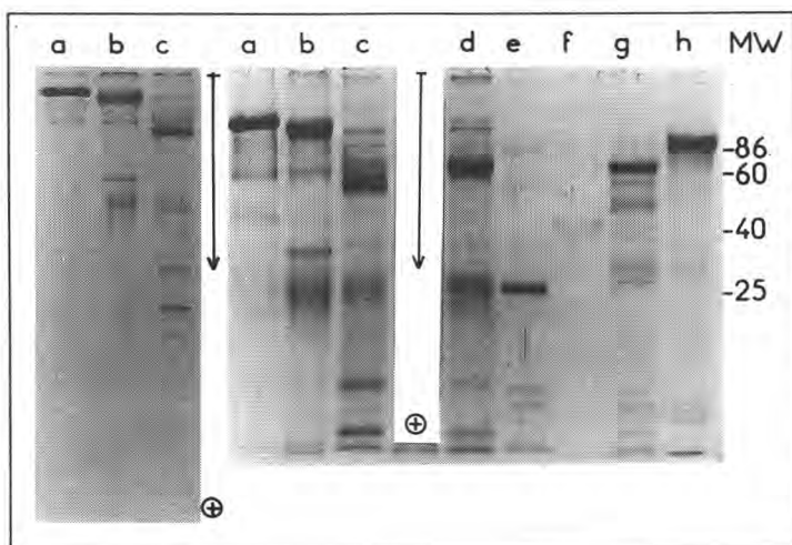
Fig 7. SDS-PAGE patterns of enzymatic preparations obtained by affinity chromatography on Lysine-Sepharose from blood (a = Plg), from whole casein (b) and from FZ (c). Slot (d) is UK-activated Plg. Standard proteins: chymotrypsinogen (e), aldolase (f), catalase (g) and bovine transferrin (h). Molecular weights in kDa.
