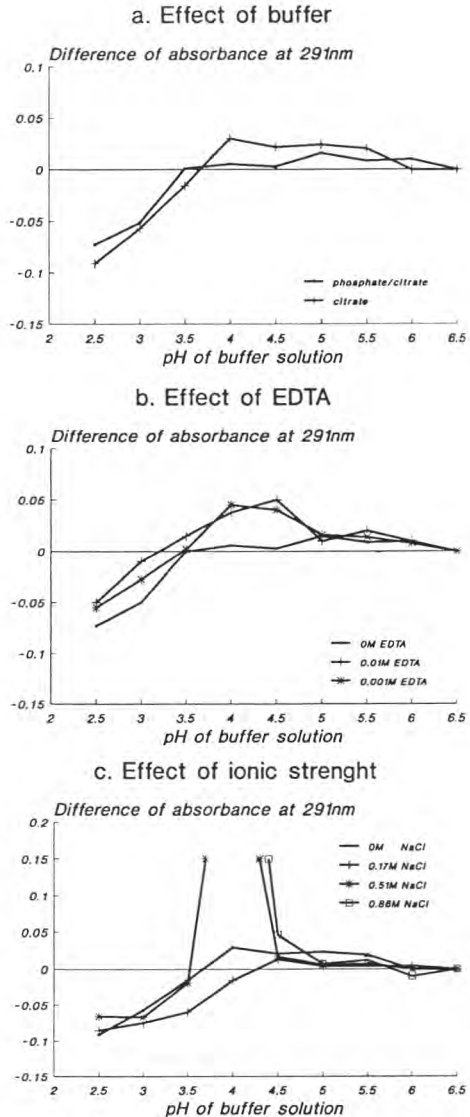
Fig. 1. Effect of buffer (a), EDTA (b) and ionic strength (c) on the change of conformation of \alpha -lactalbumin (0.08 mg/100 ml) at different pH values.
