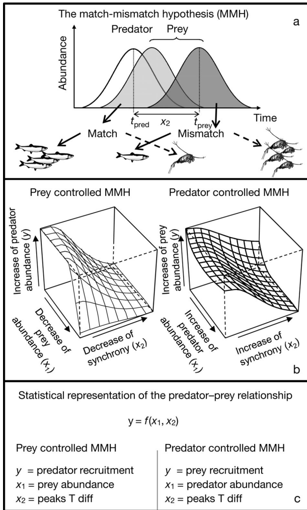
Fig. 1. The match-mismatch hypothesis (MMH) for the 2 models evaluated. (a) Cushing's (1969, 1990) MMH based on time synchrony between predator (pred) and prey (prey) ( t_{pred} - t_{prey} = x_2 , the peaks time difference, Peaks T diff). Arrows indicate opposite results for predators (solid arrows) and prey (dashed arrows). (b) MMHs with prey (left) and predator (right) control. In addition to the time component ( x_2 = Peaks T diff) prey abundance ( x_1 , left, similar to Durant et al. 2005) and predator abundance ( x_1 , right) was added. (c) The 2 statistical representations of the MMH, y = f(x_1, x_2) . f can be either a linear function or a nonparametric smoothing function s (see Table 1)
