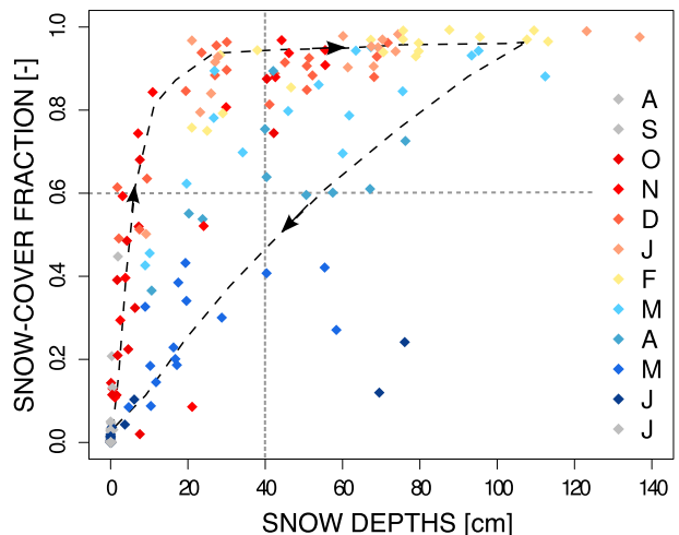
FIG. 3. MODIS SCF vs maximum mean snow-depth observations in catchment 3 over 8 days from April 2000 to March 2006. Reddish colors represent months when snow-cover accumulation prevails and bluish colors when snow-cover ablation is most important. Neutral colors such as gray and beige represent months with either no snow or very little change in the snow-cover extent.
