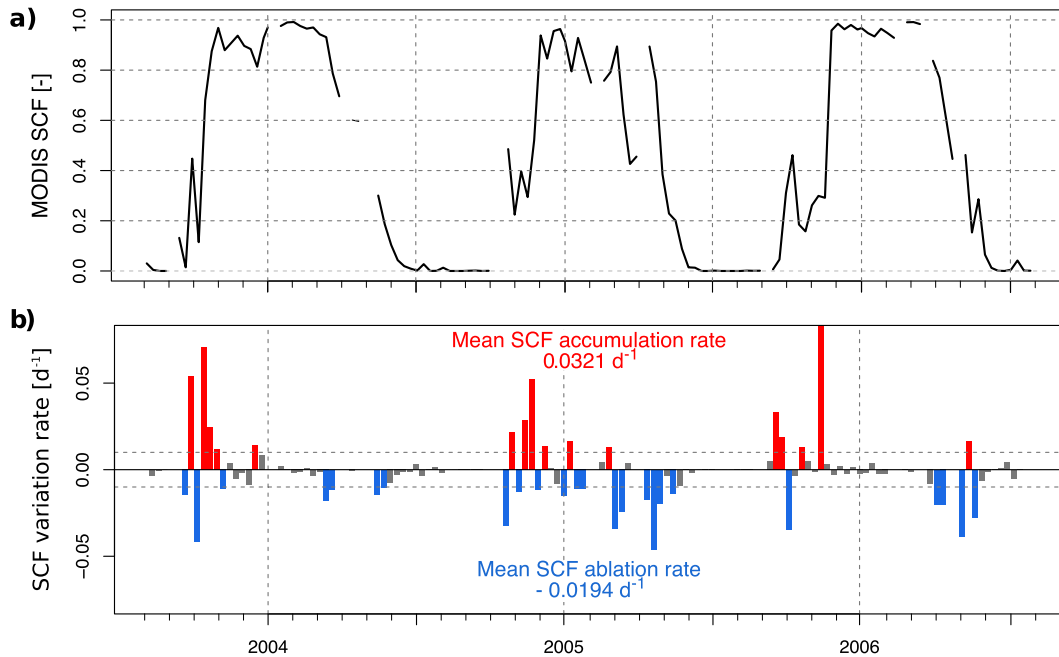
FIG. 2. (a) SCF time series extracted from MODIS images (MOD10A2) in catchment 3 from July 2003 to August 2006. Interruptions reflect weeks when cloud cover was >10\% . (b) Rates of SCF ( \text{day}^{-1} ) with accumulation represented by red bars and ablation by blue bars calculated over 2000–11. Rates <0.01 \text{ day}^{-1} in absolute terms (gray) are considered to be neutral and are not used in calculating the means. Taking them into account does not change our overall conclusion.
