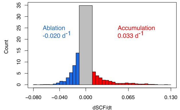
FIG. 4. Histogram of observed SCF variation rates derived from MODIS images for the entire upper Durance catchment. Mean accumulation and ablation rates (red and blue, respectively) are calculated over 2000–11. The central bin, corresponding to small absolute variation rates ( <0.01 \text{ day}^{-1} ), is in gray and not used to calculate the mean rates of accumulation or ablation. These small rates are not significant given the accuracy of MODIS images and retaining them does not change the difference between the two mean rates.
