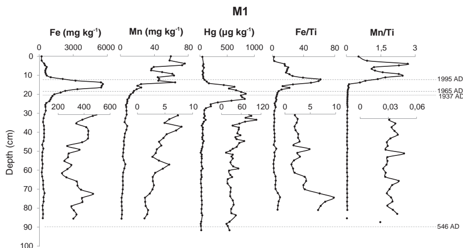
Fig. 5. Concentrations of Hg ( \mu\text{g kg}^{-1} ), Mn ( \text{mg kg}^{-1} ) and Fe ( \text{mg kg}^{-1} ), Fe/Ti and Mn/Ti ratio for the M1 core. Note that the maximum in Hg concentrations corresponds to minima in Fe/Ti in M1 core.
