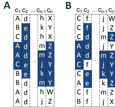
Fig. 3. Example of similar (but not identical) patterns in the annotations of two different dialogues, (A) and (B). The encoding matrices are composed of n columns. Each column has its own alphabet. The colored parts represent the two versions of the pattern which differ by an insertion/deletion, 2 gaps and 2 substitutions.
