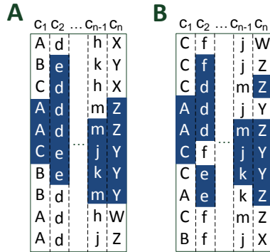
Fig. 3. Example of similar (but not identical) patterns in the annotations of two different dialogues, (A) and (B). The encoding matrices are composed of n columns. Each column has its own alphabet. The colored parts represent the two versions of the pattern which differ by an insertion/deletion, 2 gaps and 2 substitutions.
