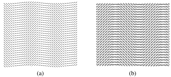
Figure 19: The concept of a tensor field (b) generalizes the notion of a vector field (a). The topological space used here is the two-dimensional Euclidean space, where each tensor is represented by (a) an arrow for a first order tensor of T^{(1,0)}(\mathbb{R}^3) and (b) an ellipsoid for a second-order tensor of T^{(1,1)}(\mathbb{R}^3) .
