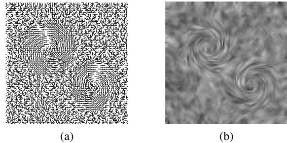
Figure 18: Some possible representations of a first-order tensor field: (a) Representation by a set of icons (arrows). (b) An image whose intensity varies with the strength and direction of smoothing of a random image using line integral convolution (LIC) (Cabral and Leedom, 1993; Stalling and Hege, 1995; Tschumperlé and Deriche, 2005).
