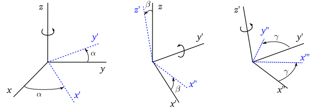
Figure 21: Rotation with Euler angles (\alpha, \beta, \gamma) in the zyz configuration. From left to right: rotation around the axis z , y' and z'' . The axes after rotation are shown in dotted lines.
