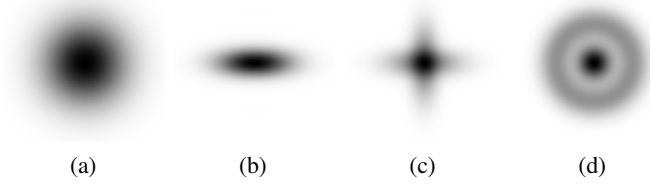
Figure 5: Examples of local diffusion profiles E observed in the brain matter measured by dMRI. The data are represented here as volumetric images 64 \times 64 \times 64 , where the center of the q -space \mathbf{q} = 0 is the center of each image. (a) Free isotropic Gaussian diffusion. (b) Restricted diffusion due to the presence of a single fiber bundle. (c) Restricted diffusion in the presence of two fiber bundles in a crossing configuration. (d) Restricted diffusion which is isotropic in direction, but has a multi-Gaussian profile radially.
