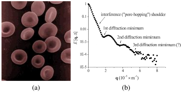
Figure 10: A plot of the radial diffusion in an environment composed of red blood cells. It is important to note that the radial decay is not Gaussian, but a “diffusion-diffraction” pattern occurs (Callaghan et al., 1991; Cory and Garroway, 1990; Kuchel et al., 1997; Regan and Kuchel, 2003) where the position of the minima are related to cell size and extracellular average size. (a) A micrograph of red blood cells (adapted from Noguchi, Rodjers and Schechter, NIDDK, under free licence). (b) Signal intensity E as a function of q (adapted from (Regan and Kuchel, 2003).)
