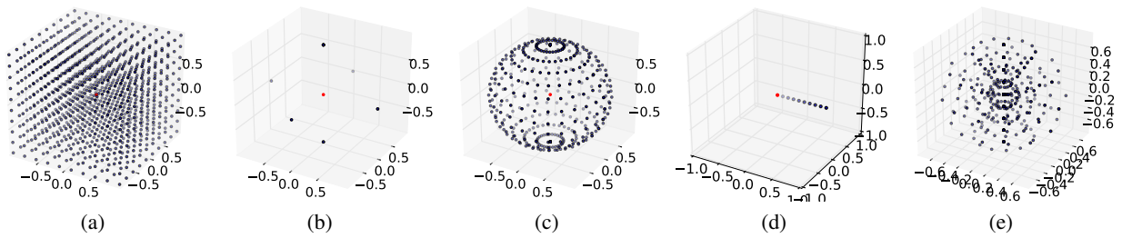
Figure 6: The analysis of the diffusion signal is closely related to the sampling of the q -space. (a) Full sampling of the q -space is currently impractical in vivo due to the significant acquisition time it would imply. (b) Low angular resolution sampling used in DTI. (c) High angular resolution sampling (HARDI). (d) Radial only sampling used in diffusion NMR. (e) Sparse sampling which combines radial and angular measurements.
