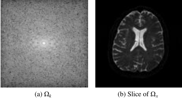
Figure 2: Acquisition of a slice of the MRI image. (a) Acquisition is done in the k -space on a slice-by-slice basis. (b) Module of the Fourier transform of the image (a).
