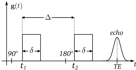
Figure 3: Pulsed Gradient Spin Echo (PGSE) sequence proposed by Stejskal and Tanner (1965). The echo formation, resulting in the diffusion signal, is acquired at the echo time TE after the 90^\circ and 180^\circ radio-frequency pulses.
