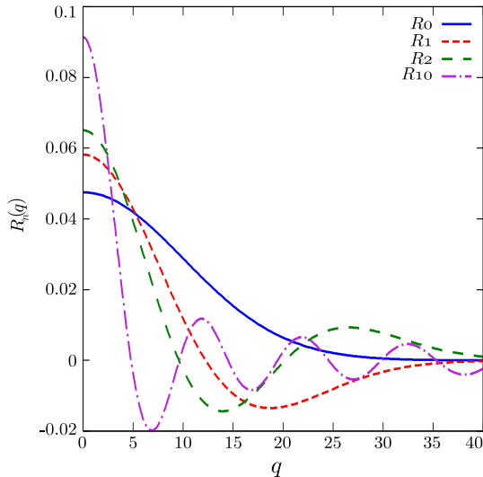
Figure 13: The first few basis functions of the radial orthonormal basis R_n , with scaling factor \zeta = 100 . Low order n functions exhibit Gaussian attenuation behaviour whereas higher order n are helpful to capture oscillating components of the MR signal.
