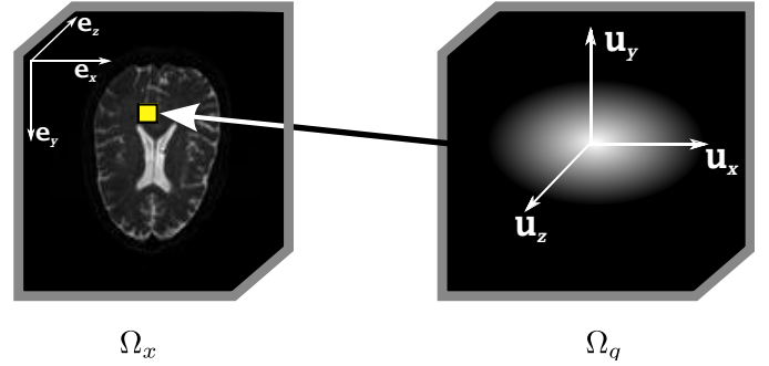
Figure 1: Our mathematical definition of the diffusion MRI image as expressed in the equation (1). Left: the position \mathbf{x} -space \Omega_x of the image, which results as the Fourier transform of the acquired k -space. Right: the diffusion q -space \Omega_q for one voxel of the \mathbf{x} -space (depicted here as a yellow rectangle).
