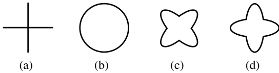
Figure 9: HARDI sampling of the diffusion signal: a schematic overview of the modeling of an intravoxel crossing of bundles nerve fibers. (a) Two fiber bundles crossing at 90^\circ inside a voxel generate a diffusion signal. (b) ADC modeling using a DTI reconstruction. (c) Generalization of the ADC modeling with HARDI sampling. The maxima of the angular profile do not match the underlying fiber bundle directions given in (a). (d) Angular feature estimation of the diffusion propagator with HARDI sampling. Adapted from (Descoteaux, 2008).
