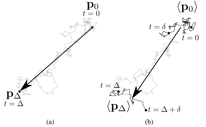
Figure 4: Simulated random walk as measured by the PGSE sequence. (a) Ideal case ( \delta \approx 0 ), (b) Real case ( \delta \neq 0 ). Adapted from (Hagmann, 2005).
