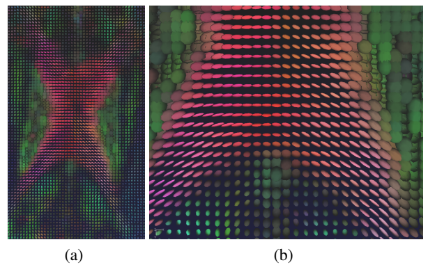
Figure 7: DTI visualization using ellipsoids: from a global to a local view. a) Visualization of the corpus callosum by a second order tensor field. b) Zoom on the bottom part of the corpus callosum. The privileged diffusion direction is the left-right axis, this is coherent since the corpus callosum links both brain hemispheres. The colours indicate the orientation of the principal eigenvector of each tensor (more details in figure 8).
