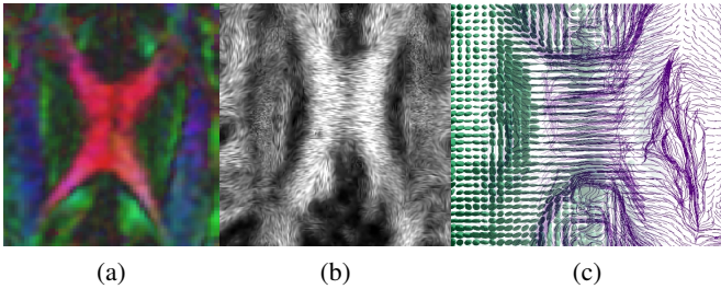
Figure 8: Some vectorial features based on the principal eigenvector of the DTI (second order tensor field). (a) The colour encodes the orientation of the vector and its norm is encoded by the brightness (red for left-right, blue for superior-anterior, green for anterior-posterior). (b) The curvature encodes the direction of each fiber and the brightness the smoothness strength. (c) Fibertracking: A visualization of nerve fiber bundles as three dimensional curves overlaid on the diffusion ellipsoids. These images are adapted from (Tschumperlé, 2002).
