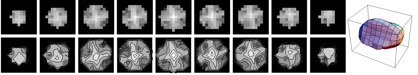
(a) First row: The raw diffusion data E[\mathbf{q}] visualized as consecutive 2D planes of the q -space. Second row: The iso-contours in two dimensions. Right: An iso-surface in three dimensions.
