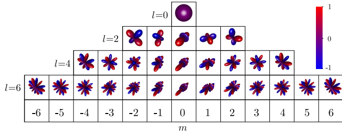
Figure 20: The real and symmetric spherical harmonics (SH) for orders l = 0, 2, 4, 6 . Blue indicates a negative value and red a positive value. The SH are normalized to lie in the range [-1, 1] .
