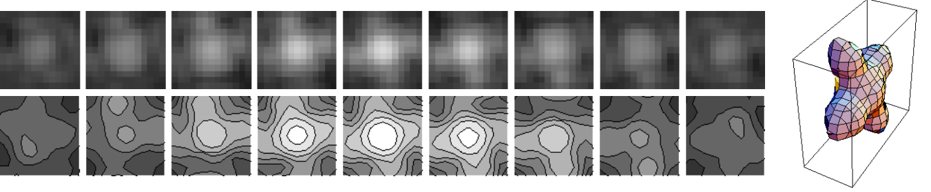
(b) First row: The diffusion propagator P[\mathbf{p}] reconstructed with the Fourier transform of E and visualized as consecutive 2D planes of the q -space. Second row: Iso-contours in two dimensions. Right: An iso-surface in three dimensions.
