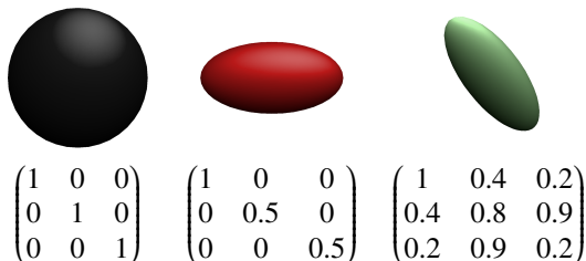
Figure 17: Examples of second-order diffusion tensors and their corresponding matrices. From left to right: isotropic diffusion, diffusion that is dominant in the direction of the X axis; and diffusion in an oblique direction.
