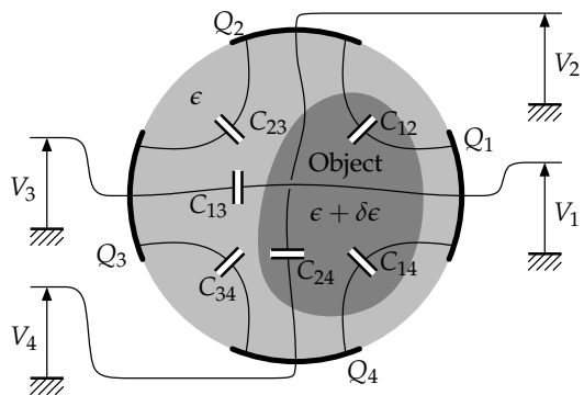
Figure 1. Simple Electrical Capacitance Tomography sensor showing all inter-capacities C_{ij} between the 4 electrodes of the sensor. The nominal permittivity is \epsilon and the object permittivity is \epsilon + \delta\epsilon .
