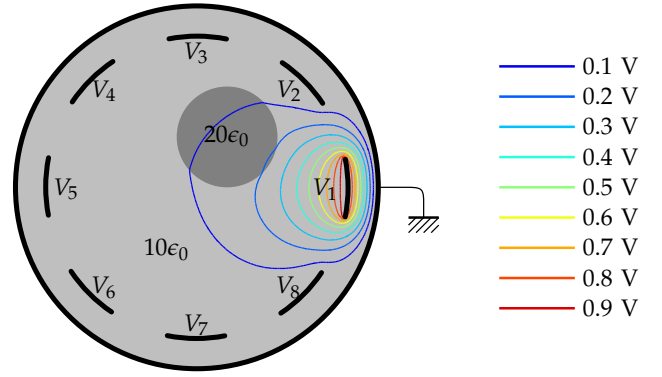
Figure 2. Example of one of the simulated situations with all electrodes grounded except V_1 = 1 V. The sensor radius is 10 cm and the object permittivity is twice the nominal one.
