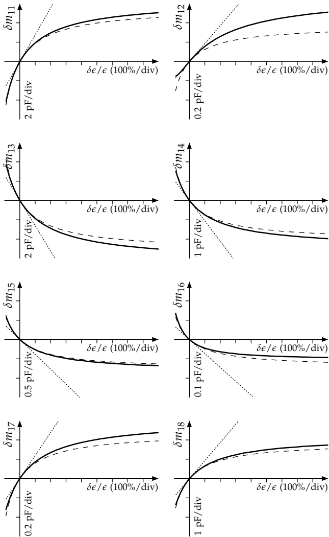
Figure 3. Variation of the first 8 measurements as a function of the relative permittivity variation \delta\epsilon/\epsilon (solid line) along with the linear model (dotted line) and non-linear model (dashed line).
