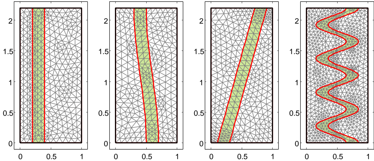
Figure 3: Meshes \#1 associated with the domains q_{T=2.2}^i : i = 0, 1, 2, 3 from left to right.
