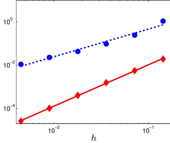
Figure 6: Example EX1 ; r = 10^{-1} ; q_T = q_{2,2}^2 ; Norms \|v - v_h\|_{L^2(Q_T)} (●) and \|y - \lambda_h\|_{L^2(Q_T)} (◆) vs. h .
