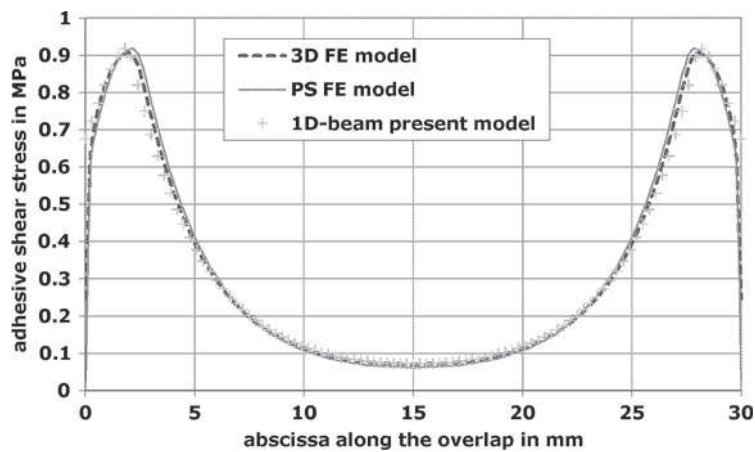
Figure 17. Comparison of the adhesive shear stress distribution along the overlap between the 1D-beam present and PS and 3D FE models, on a balanced structure.
