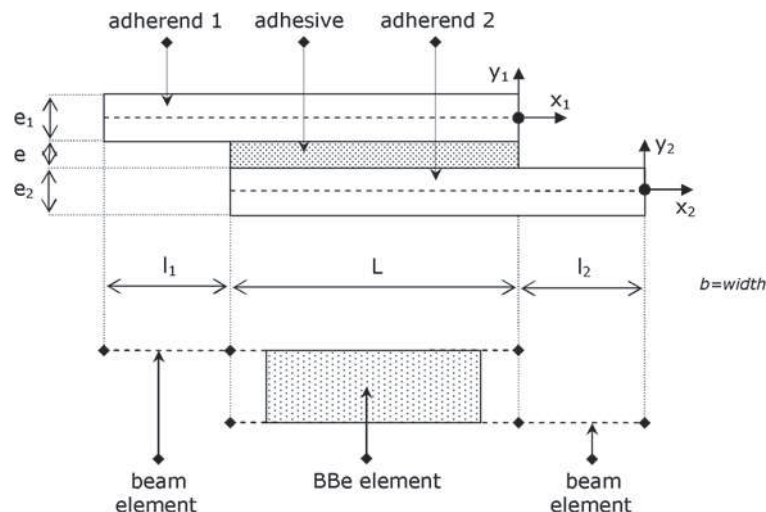
Figure 1. Idealization of a single-lap bonded joint with beam and BBe elements, for example. The dotted line corresponds to the neutral axis. Geometrical and mechanical parameters.
