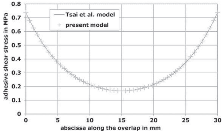
Figure 5. Comparison of the adhesive shear stress distribution along the overlap between the present 1D-bar model with the analysis provided by Tsai and Morton [16].
