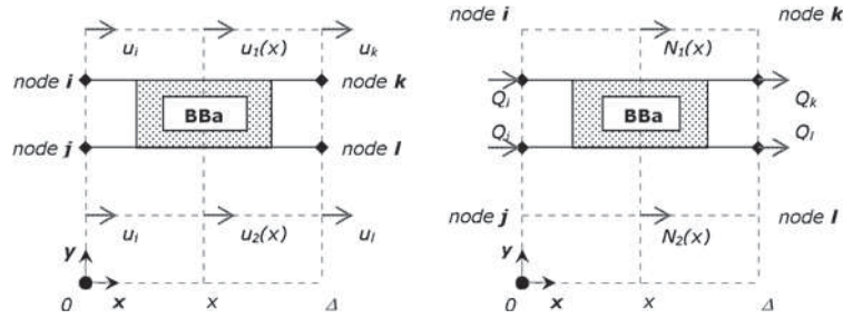
Figure 3. Displacements and forces on a BBa element.
