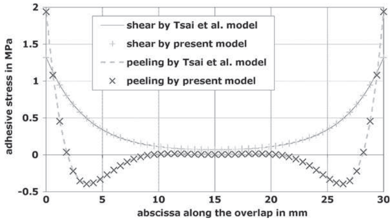
Figure 9. Comparison of the adhesive shear stress distribution along the overlap between the 1D-beam present model and the analysis provided by Tsai and Morton [16].
