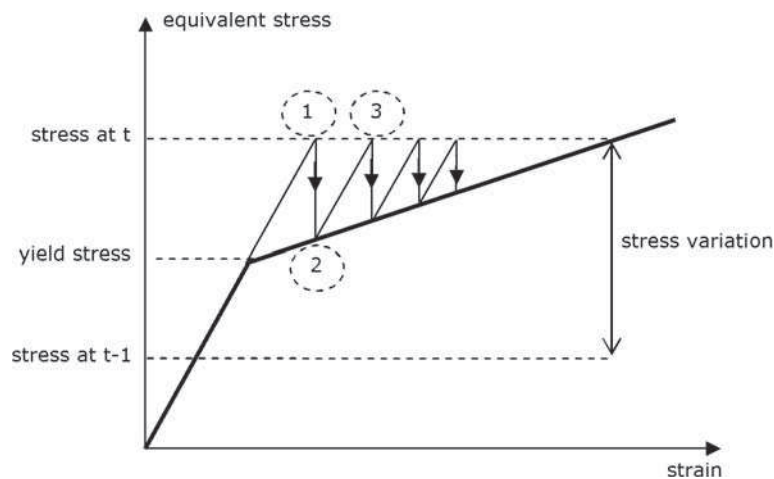
Figure 10. Principle scheme of the resolution algorithm for the elasto-plastic problem.
