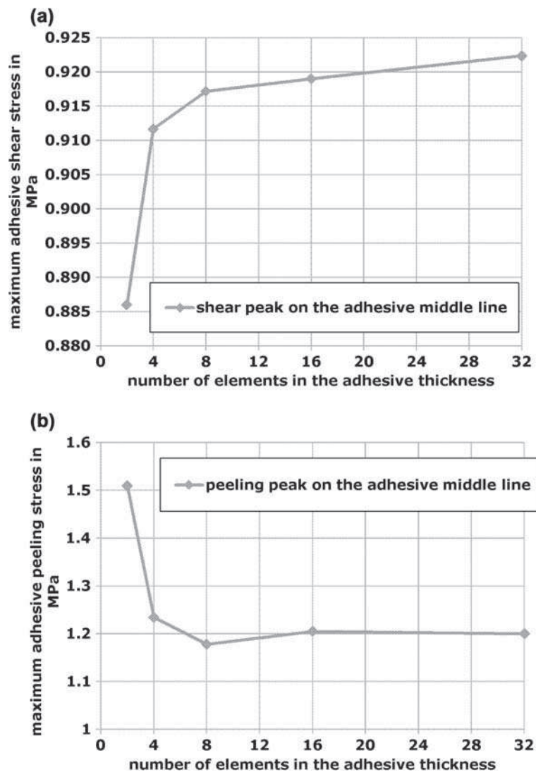
Figure 13. Shear (a) and peeling (b) peaks on the adhesive middle line as a function of the number of elements in the adhesive thickness.
