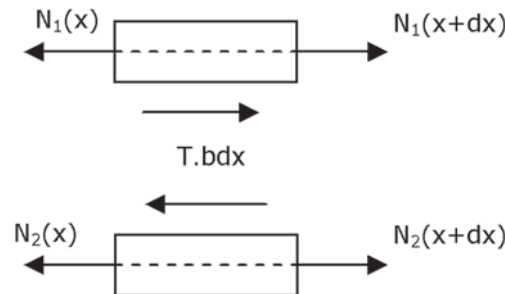
Figure 2. Free body diagram of elements of the overlap.
