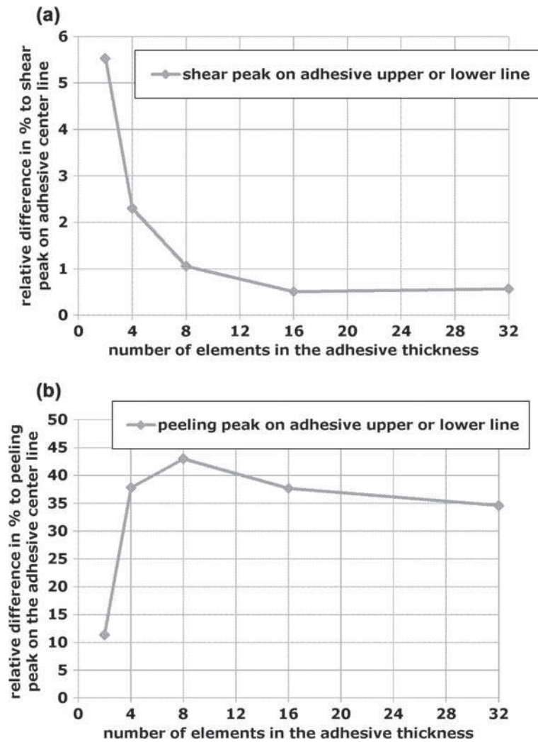
Figure 14. Shear (a) and peeling (b) peaks on the adhesive upper (or lower) line compared to the shear (a) and peeling (b) peak on the adhesive center line, as a function of the number of elements in the adhesive thickness.
