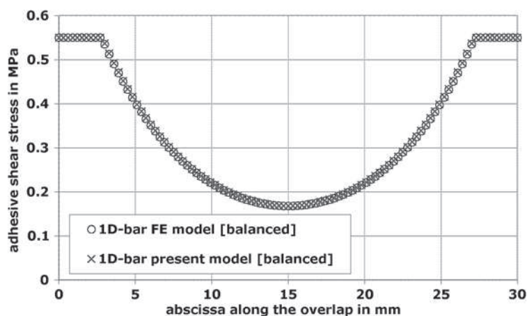
Figure 15. Comparison of the adhesive shear stress distribution along the overlap between the 1D-bar present model and 1D-bar FE models, on a balanced structure.
