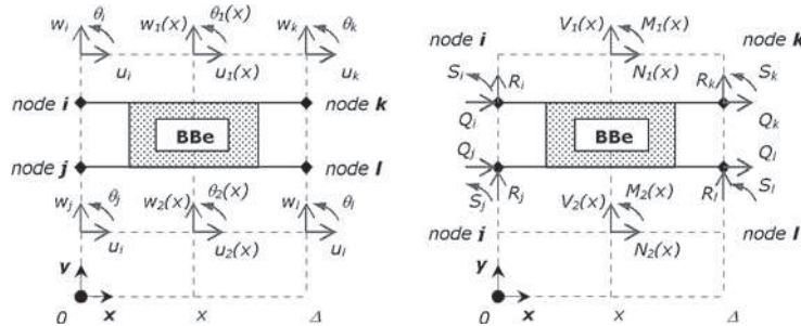
Figure 7. Displacements and forces on a BBe element.
