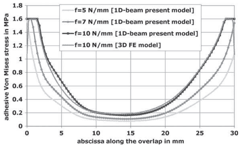
Figure 22. Comparison of the adhesive von Mises stress distribution along the overlap between the 1D-beam present model and PS and 3D FE models, on an unbalanced structure. The distributions at various intermediated applied forces are shown.
