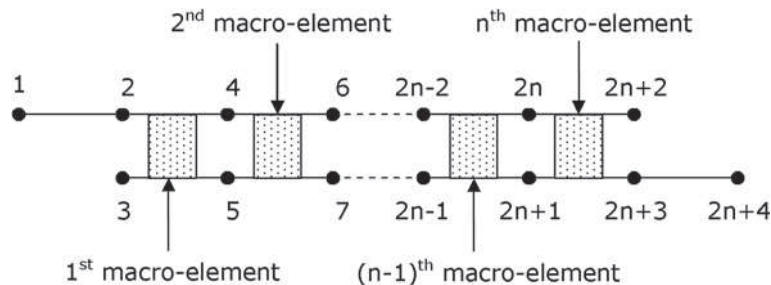
Figure 11. Numbering of the nodes on the single-lap joint meshed.
