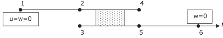
Figure 8. Bonded assembly and boundary conditions.
