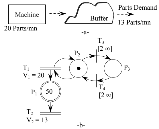
Figure 1.a. A producer consumer system; b. The D-elementary hybrid PN model of the producer consumer system;
