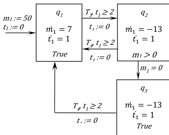
Figure A3. Hierarchical form of the hybrid automaton
