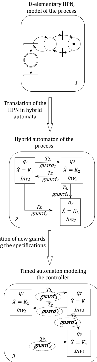
Figure 3. Controller synthesis approach
