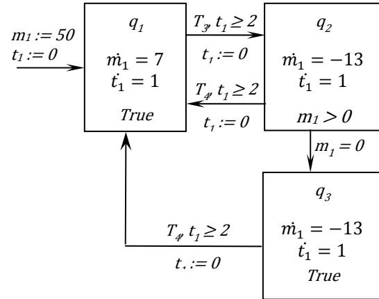
Figure 4. Hybrid automaton resulting from the translation of the D-elementary HPN in figure 1.b.
