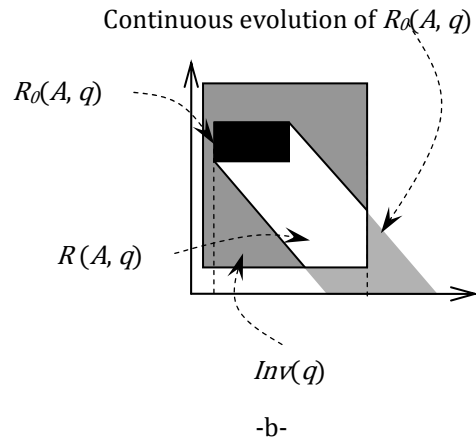
Figure 5.a) a location q from the elementary hybrid automaton, b) reachable state space in location q .
