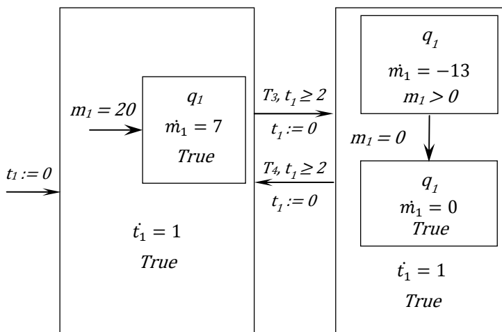
Figure A3. Hierarchical form of the hybrid automaton
