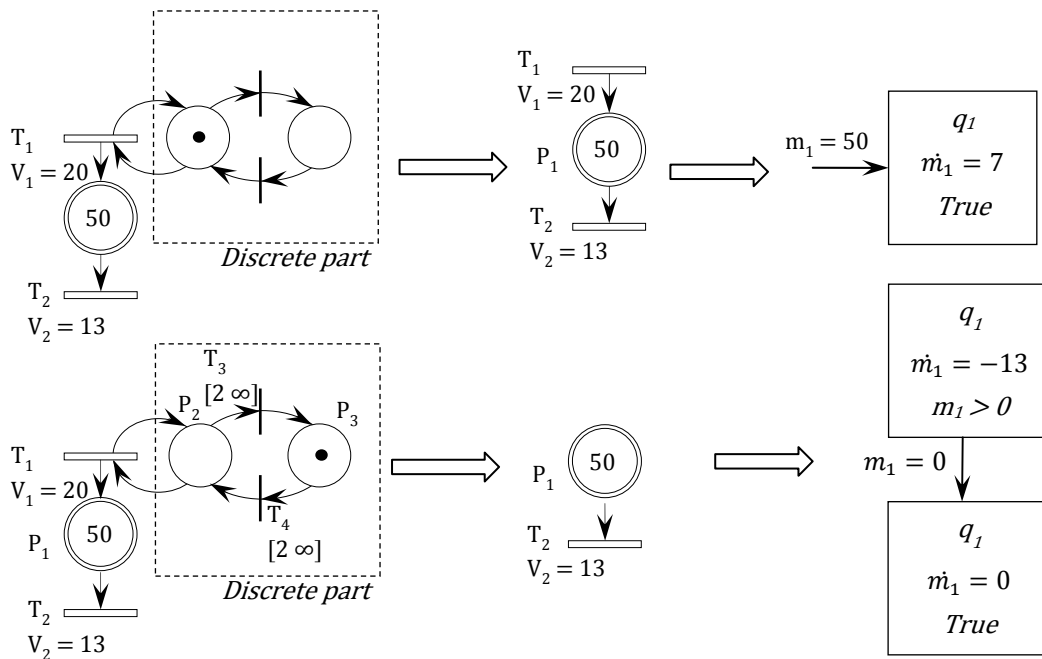
Figure A2. Continuous behaviour corresponding to each discrete marking.
