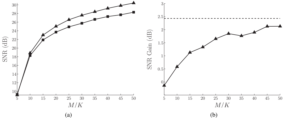
Fig. 2: Stabilized versus unstabilized reconstruction using \text{GBPND}(\ell_{2, \mathbf{w}}) and \text{BPDN} respectively. (a) The reconstruction SNR using stabilized (triangles) and unstabilized (squares) methods. (b) Observed (triangles) and theoretically predicted (dashed) SNR gain at 2.43 dB brought by stabilization.
