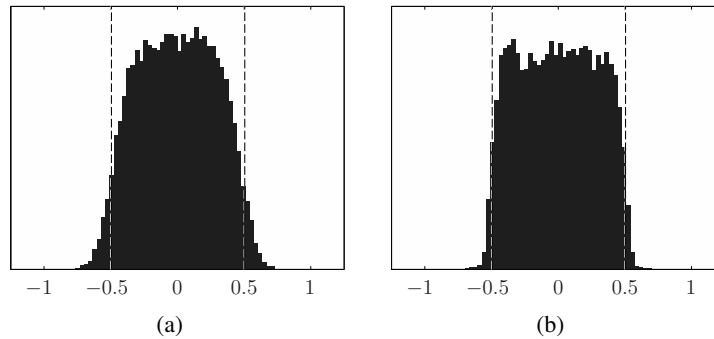
Fig. 4: Testing the Quantization Consistency (QC). (a) Histogram of the components of \alpha^{-1}(\mathcal{G}(\Phi \mathbf{x}^*) - \mathcal{G}(\mathbf{y})) for p=2 and M/K=40 (averaged over 100 trials). (b) Same histogram for p=10 . The QC is better respected in this case.
