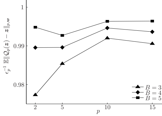
Fig. 1: Comparing the theoretical bound \epsilon_p to the empirical mean estimate of \mathbb{E}\|\mathcal{Q}_p[\mathbf{z}] - \mathbf{z}\|_{p,w} using 1000 trials of Monte-Carlo simulations, for each B = 3, 4, 5 .
