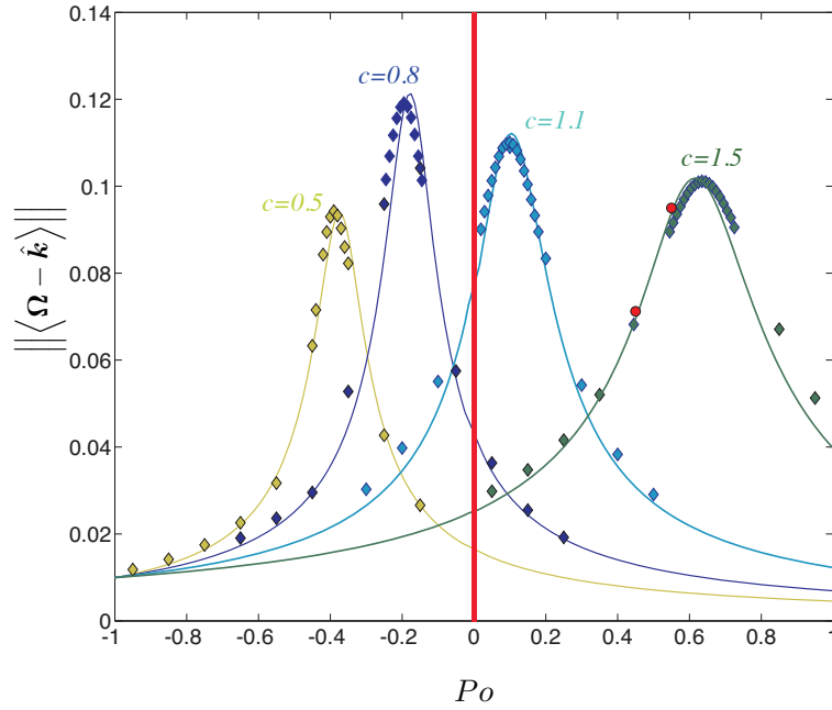
FIGURE 6. Amplitude of differential rotation, \|\mathbf{\Omega} - \hat{\mathbf{k}}\| , as a function of the Poincaré number. The symbols represent our numerical simulations at E = 10^{-3} and Ro = 10^{-2} , the solid lines represent the reduced model with the inverted values of \lambda from table 1. Each value of the polar axis c is represented by a different color as indicated. The red vertical line signifies the region of the parameter space |Po| < 10^{-2} where no \alpha can satisfy Ro = Po \sin(\alpha) . The red circles represent simulations with c=1.5 with a spatial resolution four times larger (135000 DoF).
